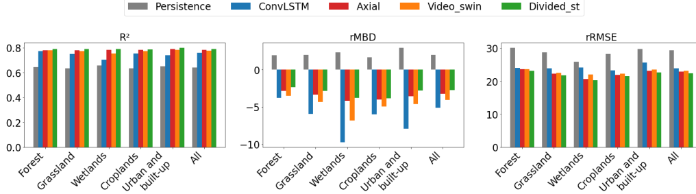
Figure 4: Performance metrics for area-based short-term forecasting under different land cover types.
