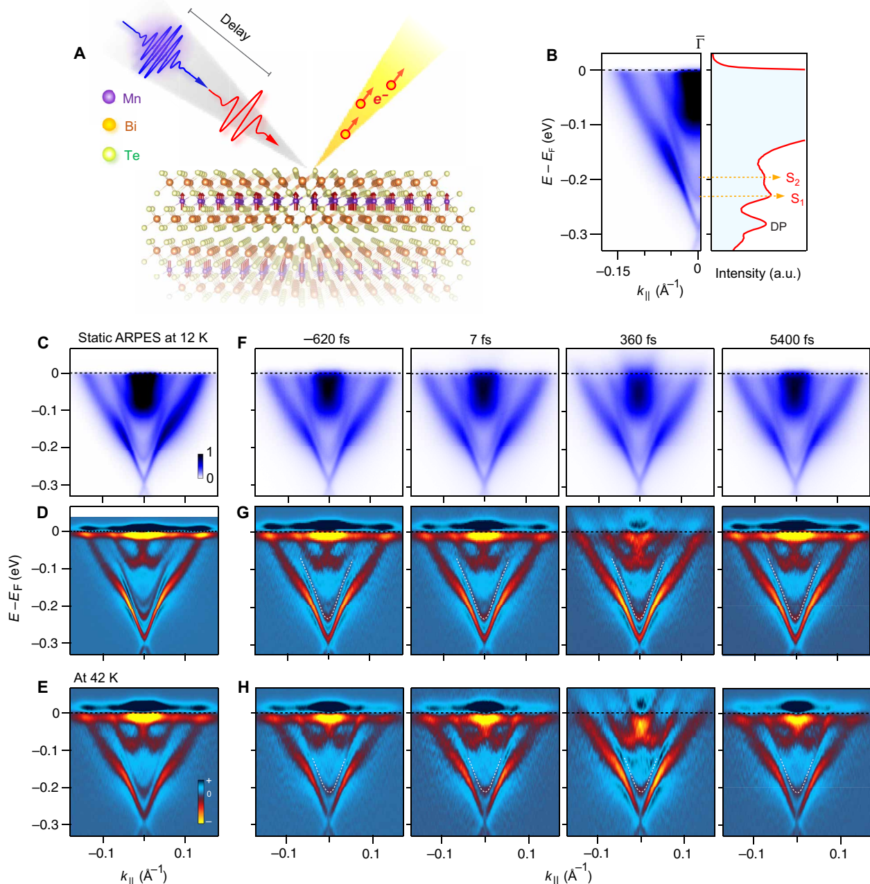
Fig. 1. Evolution of the electronic structure in MnBi 2 Te 4 (MBT) resolved by trARPES. (A) Scheme of trARPES experiment on MBT. (B) The static ARPES spectrum of MBT along the \bar{\Gamma} -K direction (left) and the energy distribution curve (EDC) taken at \bar{\Gamma} (right) with quasi-2D sub-bands S_1 and S_2 and Dirac point marked. a.u., arbitrary units. (C) Full ARPES spectrum at 12 K. Second derivative plots at (D) 12 K and (E) 42 K are also shown. (F) Time-dependent ARPES spectra at select delays and the base temperature of 12 K for an incident pump fluence of 10 \mu\text{J}/\text{cm}^2 . Time-dependent, second-derivative spectra at (G) 12 K and (H) 42 K are also shown.
