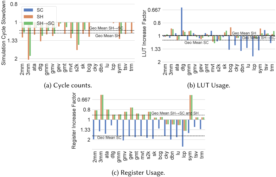
Fig. 8. Performance of Piezo designs compiled with various optimization orderings (lower is worse). Results are relative to SC → SH . The cycle counts are identical across the configurations SC and SC → SH , which is why no blue bars appear in (a).
