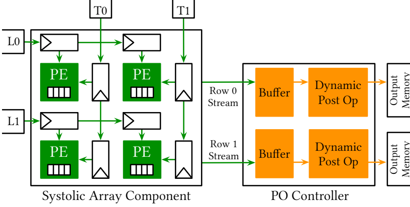
Fig. 10. Our 2 \times 2 systolic array with a dynamic post op. The buffers in the post op controller are not necessary for static post ops. Green is static and orange is dynamic. Input memories (L0, L1, T0, T1) may have non-fixed length.
