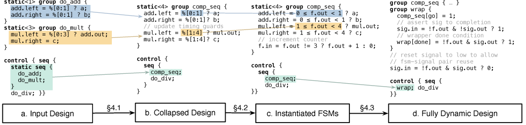
Fig. 5. The stages for implementing Piezo's static control operators.
