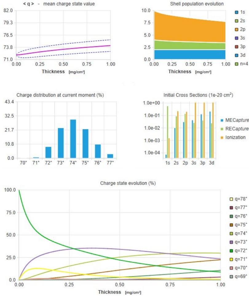
Figure 1: Charge state evolution distributions calculated by the ETACHA-GUI code for ^{207}\text{Pb}^{72+} at 28.9 MeV/u passing a carbon foil of 1 \text{ mg/cm}^2 .
