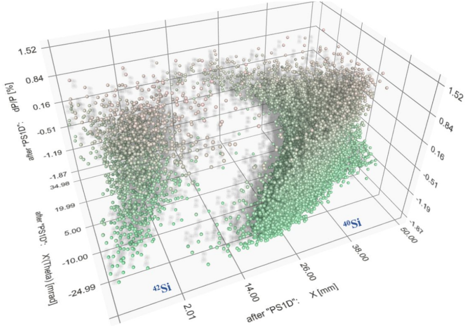
Figure 2: 3-D plots of the X , X' , dP/P distributions of ^{40}\text{Si} and ^{42}\text{Si} fragments in front of the ARIS preseparator final focal plane slits calculated by Monte Carlo method with 5^{th} order maps use in the reaction ^{48}\text{Ca}(251 \text{ MeV/u}) + ^{12}\text{C}(10\text{mm}) . The separator set to produce ^{42}\text{Si} uses a 6-mm special shape aluminum degrader located in the dispersive focal preseparator plane, which compress fragment momentum distributions by a factor 3. Calculated transmission through the next slits ( \pm 8 \text{ mm} ) are 0.03% and 87.2% for ^{40}\text{Si} and ^{42}\text{Si} , respectively.
