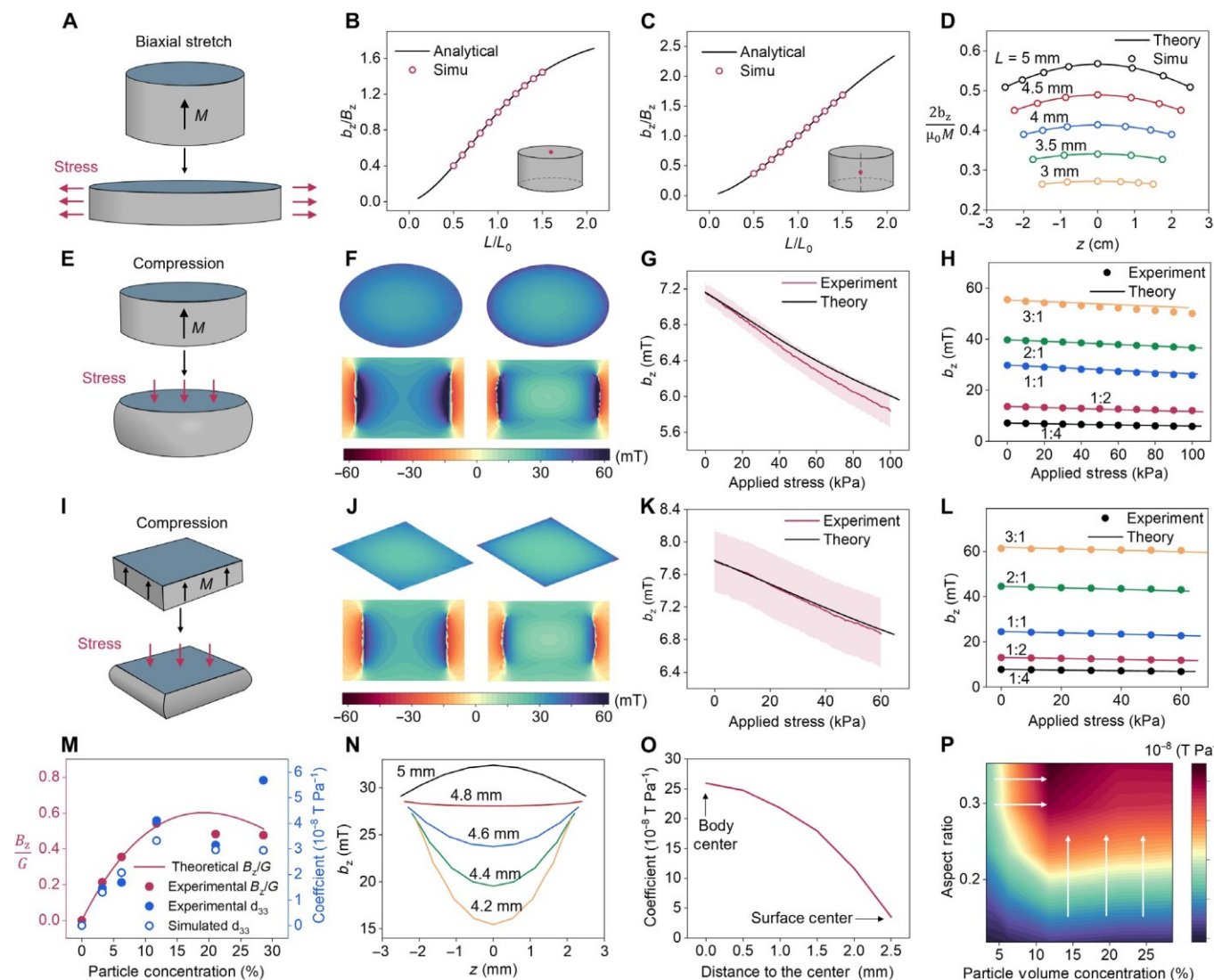
Fig. 2. Investigate the magnetoelastic effect in soft systems with a compression deformation mode. (A) Scheme of a cylindrical magnetoelastic system subject to biaxial stretch. (B and C) Simulation (Simu) result and analytical solution are consistent for the b_z at both the surface center (B) and the body center (C) under the biaxial stretch. L_0 = 5 mm. (D) Normalized b_z along the axis of the cylindrical system under various biaxial stretching conditions. (E) Scheme of a cylindrical magnetoelastic system subject to compression. (F) Simulated b_z mapping on the top surface and cross section of the cylindrical system in its initial and compressed states. (G and H) Relationship between b_z and applied stress at the surface center of the cylindrical system with different micromagnet-to-polymer weight ratios includes 1:4 (G) and the summary (H). experimental results represent the average value from three independent experiments. Shaded area represents the Sd. (I) Scheme of a cuboidal magnetoelastic system subject to compression. (J) Simulated magnetic flux density mapping on the top surface and cross section of the cuboidal system in its initial and compressed states. (K and L) Relationship between b_z and applied stress at the surface center of the cuboidal system with different micromagnet-to-polymer weight ratios includes 1:4 (K) and the summary (L). experimental results represent the average value from three independent experiments. Shaded area represents the Sd. (M) Prediction of the variation of B_z/G , a quantity that characterizes the Mc factor, with the particle volume concentration for the cylindrical system. (N) b_z along the cylindrical axis when the system is compressed from 5 to 4.2 mm. (O) the simulated Mc factors at distinct positions inside the cylindrical system. (P) Mapping of Mc factor with respect to the particle volume concentration and the aspect ratio predicted by the model.
