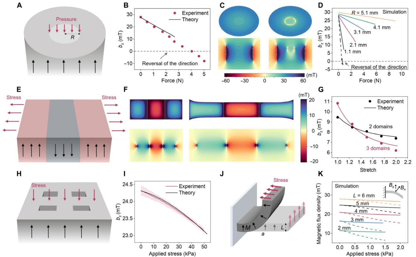
Fig. 3. Validate the universality of the framework for understanding the giant magnetoelastic effect in soft systems. (A) Scheme of a cylindrical system subjected to localized compression. (B) comparison of the experimental and simulation b_z -force relationship under local compression. (C) corresponding simulated b_z mapping on the top surface and cross section of the cylindrical system in its initial and compressed states. (D) Simulated b_z -force relationship under various local compression conditions, with the radius of deformation area ranging from 1.1 to 5.1 mm. dashed line represents the modeling results not incorporating the magnetic force. (E) Scheme of a cuboidal system with three alternating magnetization domains subjected to uniaxial stretch. (F) corresponding simulated B_z mapping on the top surface and cross section of the cuboidal system in its initial and stretched states. (G) comparison of the experimental and simulated B_z -stretch curves for cuboidal systems with two and three magnetization domains. (H) Scheme of a soft lattice-structured magnetoelastic system subjected to compression. (I) comparison of the simulated and experimental b_z -applied stress curves at the surface center of the lattice structure. experimental results represent the average value from three independent experiments. Shaded area represents the Sd. (J) Scheme of a cuboidal system subjected to bending deformation. (K) Simulated relationship between magnetic flux density and applied stress in the bent cuboidal system, with the thickness of the system varying from 2 to 6 mm. Solid lines depict the variation of b_n , while dashed lines indicate the variation of b_z .
