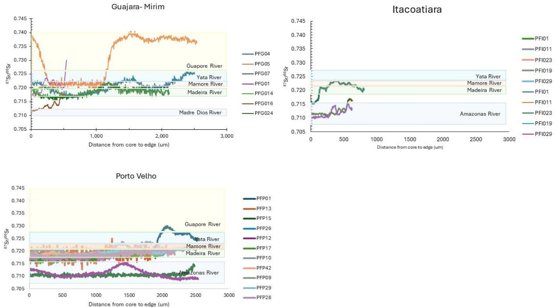
Figure 3. Sr isotopic signatures from core to edge of the otolith for P. fasciatum specimens collected in three rivers within the Amazon basin. The Sr range for each river is represented by boxes with different colors that include minimum and maximum Sr signature values for each river. Data show the Sr isotopic signatures of specimens that performed migrations between rivers with different Sr signatures in Guajara-Mirim, Itacoatiara, and Porto Velho.
