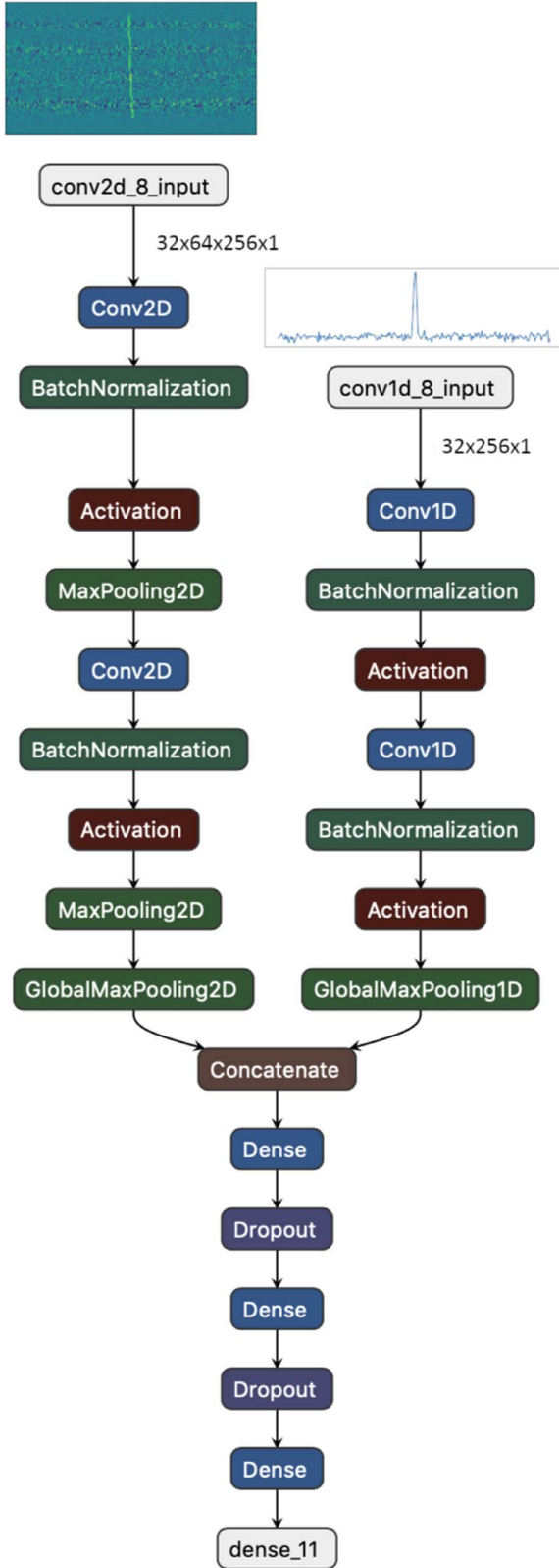
Figure A2. The neural network model architecture of the ML classifier built to identify dedispersed broadband ETI beacons. The model was trained on two different characteristics of the broadband pulse, corresponding to the two branches: the left branch is the spectrogram branch, which takes an input of a 2D dynamic spectrum, while the right branch takes an input of a 1D time series. Both branches were concatenated to assess final probability (see Appendix A.2 for details).
