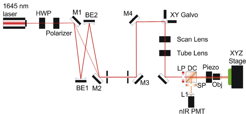
Figure 2. Schematic of the NIR-II two-photon microscope. Schematic of the dual NIR excitation-emission two-photon microscope for imaging through highly scattering media. Mirror pairs M1:M2 and M3:M4 are used to align the left and right halves of the light path, respectively, to the two alignment apertures between M2 and M3. M1 can be adjusted to bypass the beam expansion mirrors. BE: beam expander, LP: 1500 nm longpass filter, SP: 1500 nm shortpass filter, DC: dichroic mirror comprising 1500 nm longpass and 850 nm shortpass, Objective: 20x Leica, with 2.0 mm working distance and numerical aperture of 0.95.
