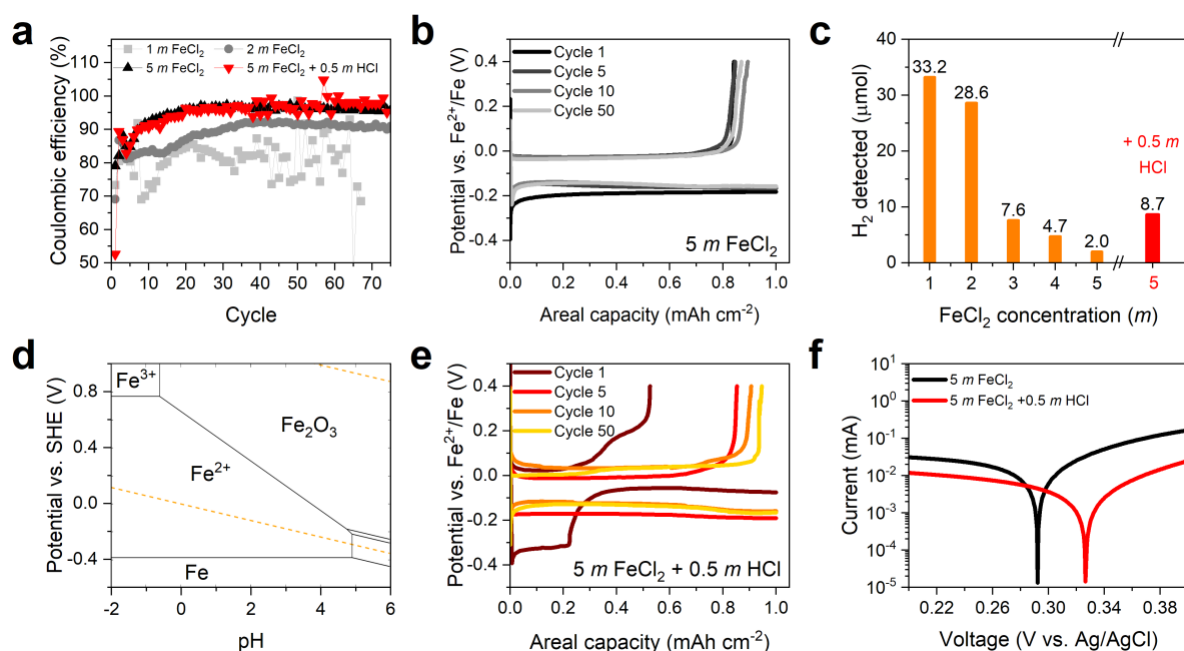
Figure 1. The electrochemical performance of FeMA in \text{FeCl}_2 electrolytes of various concentrations. (a) CE of the FeMA measured in three-electrode cells with a Ti foil working
