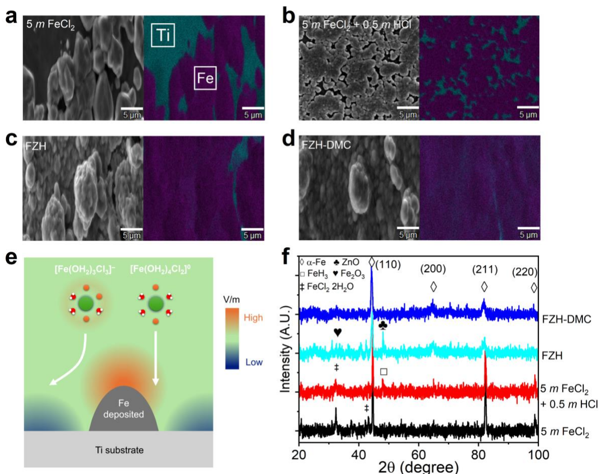
Figure 5. SEM images of the plated mass on a Ti current collector, taken after the 10 th discharge using electrolytes of (a) 5\text{ m FeCl}_2 , (b) 5\text{ m FeCl}_2 + 0.5\text{ m HCl} , (c) FZH, and (d) FZH-DMC. (e) Schematic illustration of the electric field distribution around the deposited iron mass and its effect on the ferrous ions with different solvation structures. (f) XRD patterns of the electrodes after the 50 th discharge using various electrolytes.
