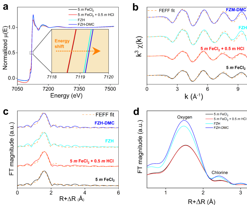
Figure 4. XAS measurements using synchrotron light source. (a) Normalized Fe K-edge XANES with an inset of the energy shift at \frac{1}{2}\mu(E) in concentrated chlorine electrolytes, (b) the k^3 -weighted Fe K-edge EXAFS spectra, and (c) their corresponding Fourier Transform (FT) magnitude of the electrolytes (solid line – experimental results, orange dashed line – best FEFF fits of the EXAFS model in the R range of 0.5 - 5\text{ \AA} ). (d) FT magnitude of the electrolytes overlapped.
