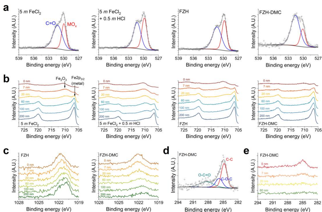
Figure 6. XPS profiles of anode after 50 th discharge with various electrolytes. (a) Peak deconvolution results of the O 1s spectra. Depth profiling of (b) Fe 2p and (c) Zn 2p spectra. (d) Peak deconvolution results of the C 1s spectra and (e) depth profiling of the C 1s spectra for FZH-DMC samples.
