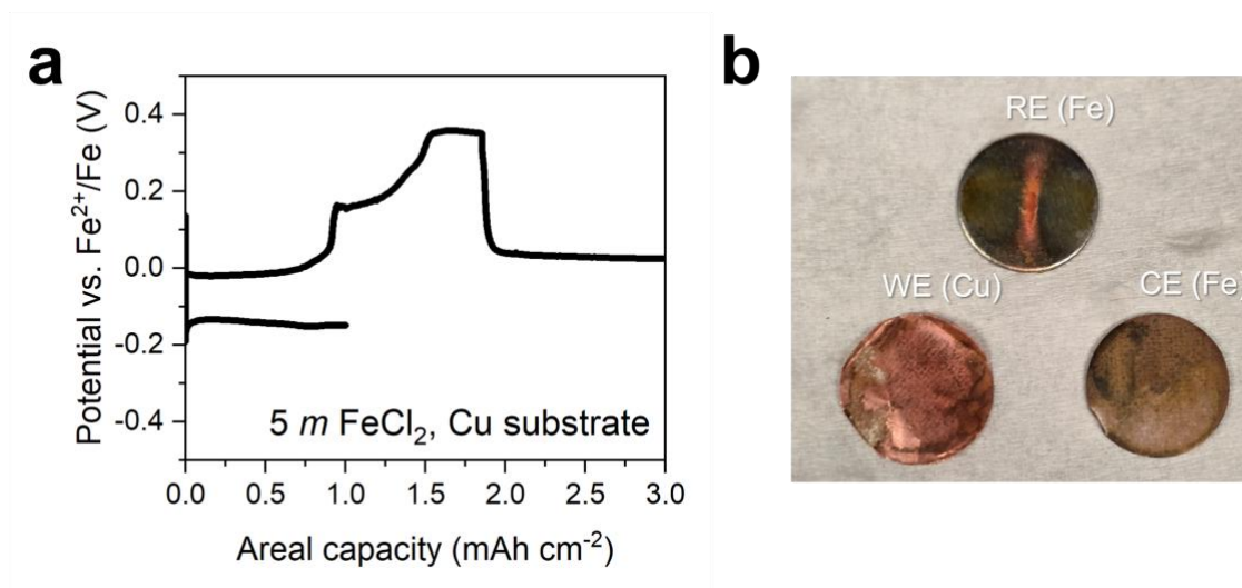
Supporting Figure S1. Impact of the Cu current collector material on the CE measurements. (a) GCD profiles of the Fe anode using Cu foil as a working electrode current collector. (b) Digital images of electrodes taken out from the Swagelok cell after observing “endless” charging of the cell.
