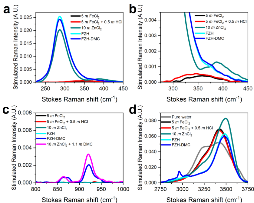
Figure 3. Ground-state FSRS spectra of various electrolytes in the (a) low-frequency region showing ion clusters, (b) enlarged view of the hydrated cluster region, (c) mid-frequency region depicting water-DMC interactions, and (d) high-frequency region of the H-bonding network of water.
