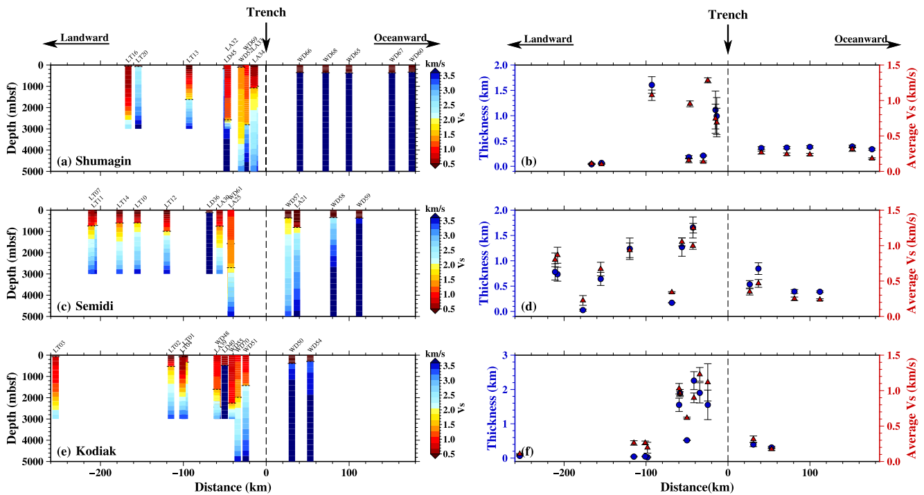
Figure 10. The 1-D S-wave velocities, as well as sediment thickness and depth-averaged Vs of seafloor sediment beneath each station, showing along dip. (a)–(b) Shumagin segment. (c)–(d) Semidi segment. (e)–(f) Kodiak segment.
