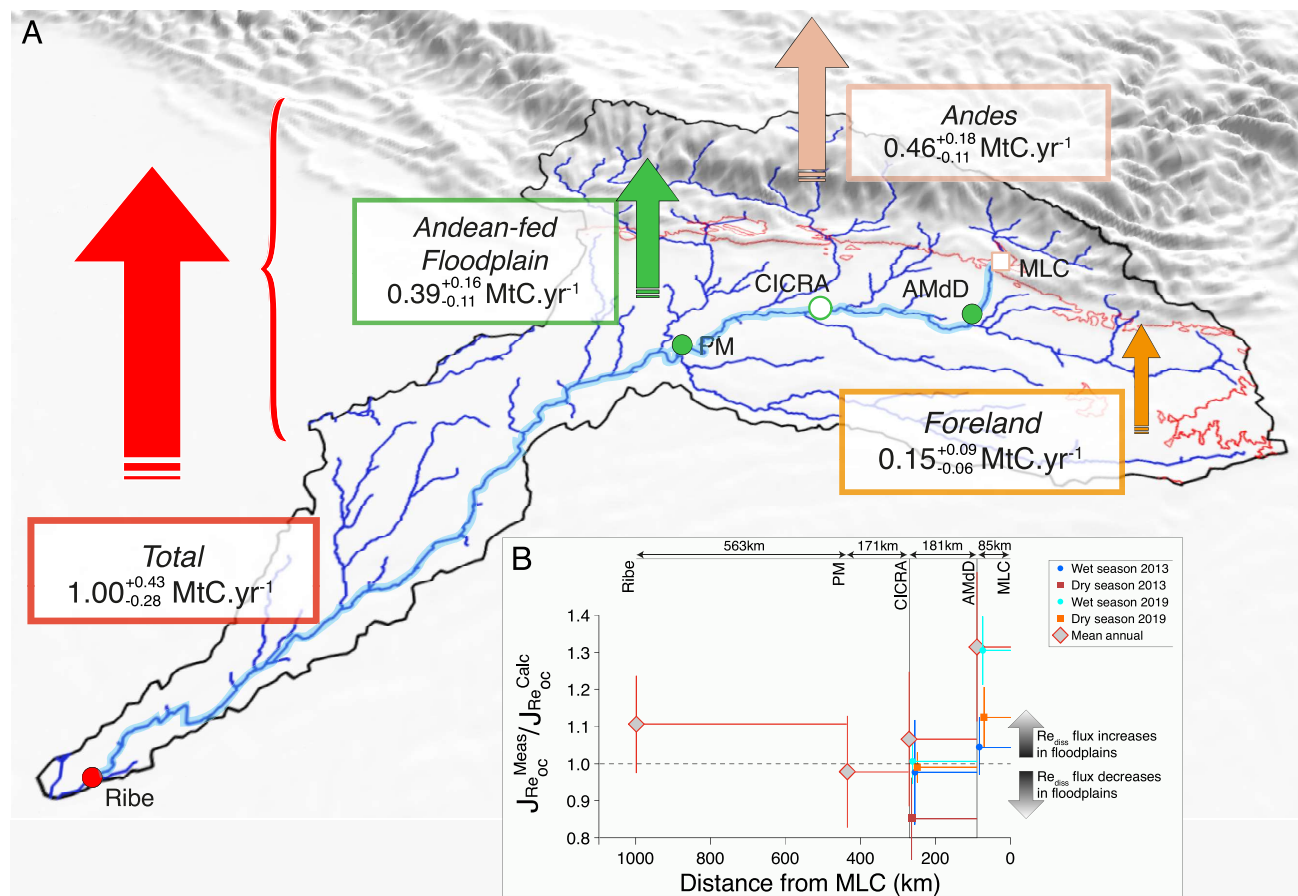
Fig. 4. (A) Estimated net contribution (vertical arrows) of each geomorphic zone to the total flux of OC_{petro} oxidation and associated CO_2 release at the scale of the whole Madre de Dios River basin. MLC = Mountain Front, AMdD = Alto Madre de Dios, PM = Madre de Dios at Puerto Maldonado, Ribe = Madre de Dios at Riberalta. The red squiggly line corresponds to the 500-m elevation contour. (B) Ratio between the measured dissolved rhenium flux derived from OC_{petro} oxidation ( J_{Re-OC}^{meas} ) and the predicted flux ( J_{Re-OC}^{calc} ) using the tributary mixing model ( SI Appendix ), as a function of the channel distance from MLC. A value >1 can be interpreted as OC_{petro} oxidation in the floodplain. Vertical bars represent the uncertainties. The studied floodplain transect corresponds to the channel highlighted in light blue on panel A.
