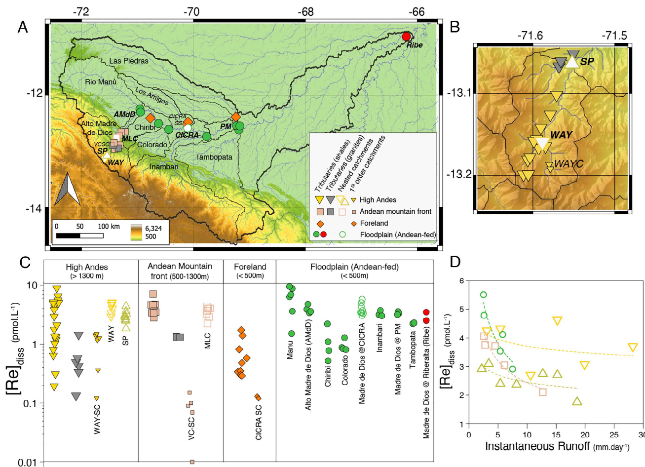
Fig. 1. (A) Map of the Madre de Dios River basin with the location of the samples from this study. (B) Inset showing the location of the samples in the High Andes. (C) [Re]_{diss} concentration (in pmol L -1 ) in the various geomorphic settings for all river samples from this study. The [Re]_{diss} from the two hot spring samples plot above the range shown on the figure (see data in Dataset S1). (D) [Re]_{diss} versus instantaneous runoff W (water discharge normalized by catchment area, mm day -1 ) at the time of sampling for the main nested catchments of this study (WAY, SP, MLC, and CICRA).
