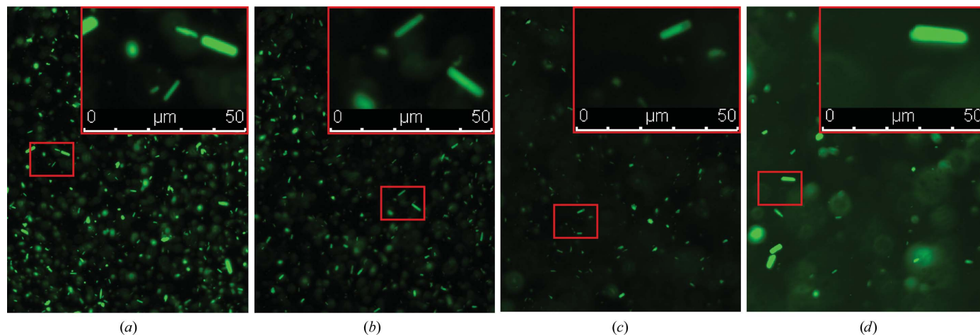
Figure 3 EGFP- \mu NS (448–605) crystals embedded in LCP. GFP fluorescence microscopic images of crystals 0 h ( a ), 24 h ( b ), 72 h ( c ) and 96 h ( d ) after mixing with LCP.
