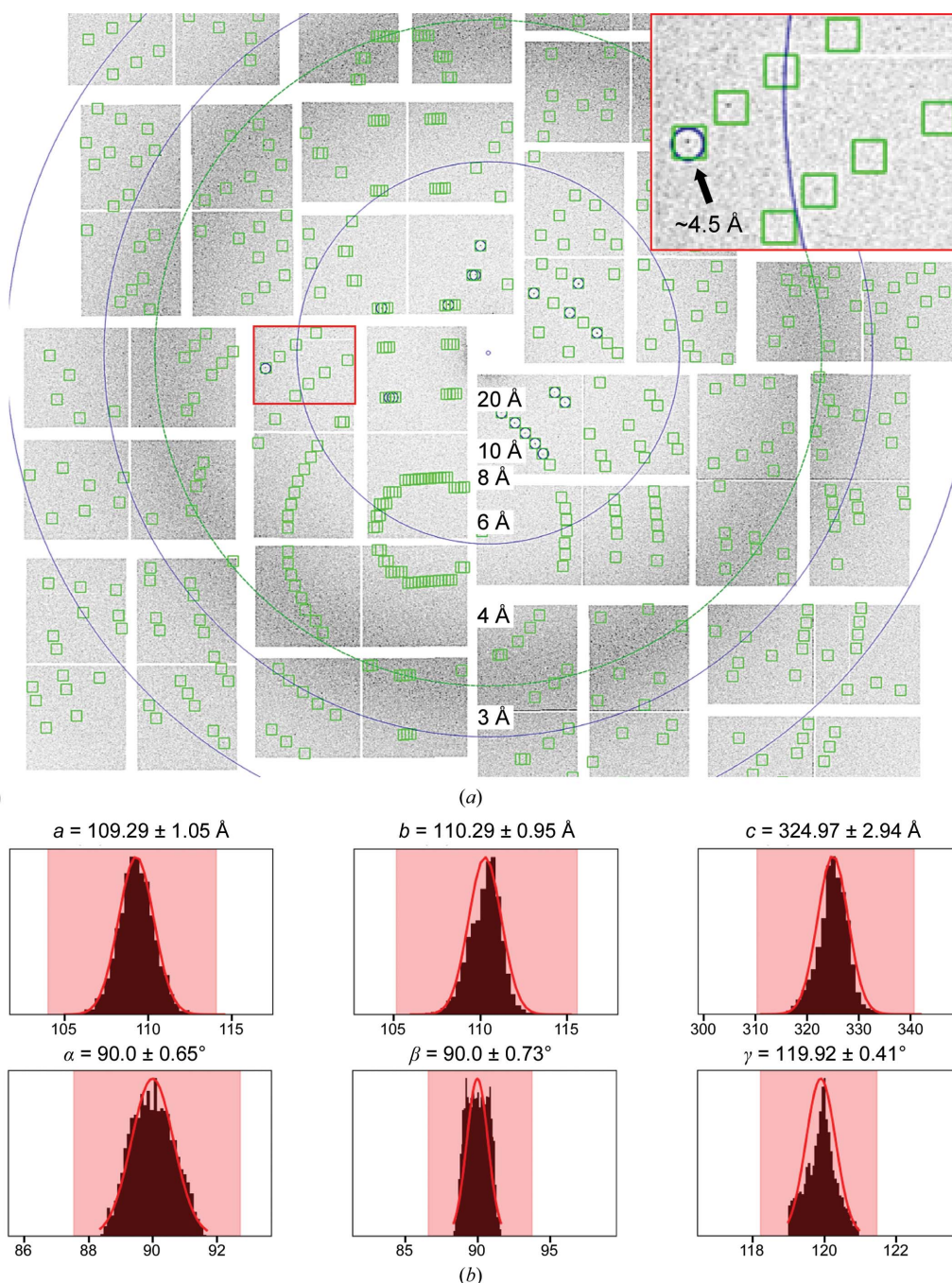
Figure 4 SFX of EGFP- \mu NS (448–605) crystals delivered in agarose. (a) Indexed diffraction pattern of a single EGFP- \mu NS (448–605) crystal. The black arrow in the inset shows a Bragg spot at about 4.5 Å resolution. (b) Unit-cell distribution of the 4227 indexed snapshots.
