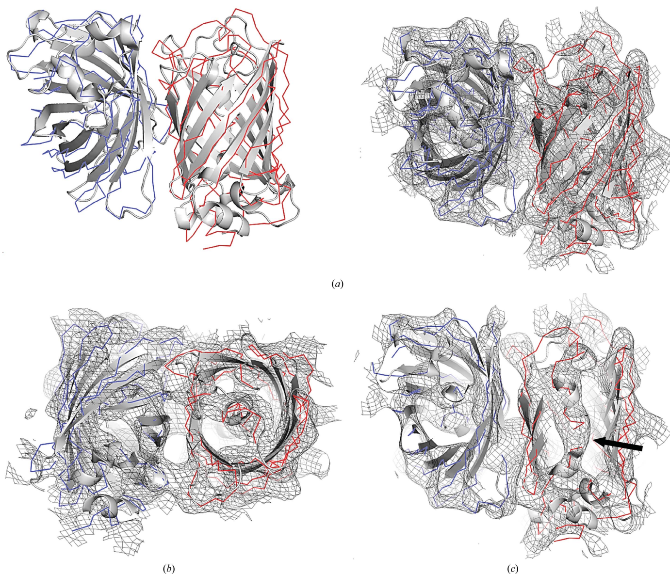
Figure 5 Electron-density maps ( 2mF_o - DF_c ) contoured at 1\sigma . (a) Ribbon representations of the two EGFP molecules in the asymmetric unit are shown without (left) and with (right) maps in the same orientation. (b) A 90^\circ rotation of the EGFP molecules shown in (a). (c) Helical fragments running through the center of one of the EGFP molecules that coordinate the fluorescent chromophore are shown and highlighted by the black arrow. For clarity, the EGFP molecules from PDB entry 3lvc have been overlaid and are represented as a light gray cartoon in all panels shown.
