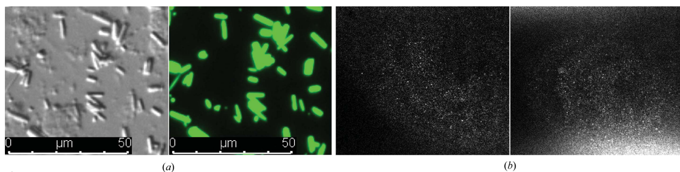
Figure 2 EGFP- \mu NS (448–605) crystals resuspended in PBS buffer. ( a ) EGFP- \mu NS crystals extracted from Sf9 cells by gentle sonication and resuspended in PBS buffer three days post-infection observed by DIC (left) and GFP fluorescence (right) microscopy with the same field of view. ( b ) SONICC images of high-density EGFP- \mu NS (448–605) crystal pellets extracted from Sf9 insect cells two days (left) and three days (right) post-infection.
