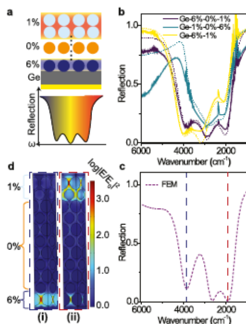
Figure 6. Cavity structure with multiple resonances by stacking different types of NCs. (a) Schematic representation of a photonic structure composed of a monolayer of highly doped (6% Sn) ITO NCs, multilayers of undoped (0% Sn) \text{In}_2\text{O}_3 NCs, and two layers of low-doped (1% Sn) ITO NCs on a Ge spacer layer. Multiple resonances are expected to appear in the reflection spectrum with distinct spatial localizations. (b) Far-field reflection spectra of cavity-coupled NC assemblies with various stacking sequences. The legend indicates the stacking sequence combinations of 6% Sn ITO, 1% Sn ITO, and \text{In}_2\text{O}_3 NCs. The dotted lines represent the reflection spectra predicted using the transfer matrix model. (c) Far-field reflection spectrum predicted using FEM for the Ge-6%-0%-1% case. (d) Near-field intensity distributions corresponding to the same configuration as in (c) for excitation at high and low resonance frequencies indicated by the dashed lines in (c).
