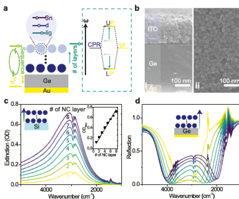
Figure 1. Design of tunable cavity-coupled NC assemblies. (a) Schematic of experimental tuning knobs, including synthetically controlled parameters of the NC composition, the thickness of the Ge spacer, the NC assembly thickness, and the stacking sequence. The properties of the upper and lower polariton (UP and LP) modes resulting from coupling between the collective plasmon resonance (CPR) and photonic modes (pt) are adjusted based on these variables. (b) Scanning electron microscope (SEM) images of eight layers of 25 nm ITO NCs on a 215 nm Ge spacer layer and 100 nm Au layer. (i) Cross-sectional and (ii) top-down images. (c) Extinction spectra of 25 nm, 2.7% Sn ITO NCs as a function of the number of NC layers on an IR-transparent silicon wafer. Spectra for one to eight NC layers are shown. The inset shows the approximately linear dependence of the peak intensity of the extinction spectrum on the number of NC layers. (d) Reflection spectra of the stacks of the same ITO NCs in a Salisbury screen configuration, composed of 160 nm Ge and 100 nm Au. The peaks around 2300 and 1600 \text{cm}^{-1} correspond to the vibrational modes of \text{CO}_2 and \text{H}_2\text{O} , respectively, due to the fluctuations in residual atmospheric gases after \text{N}_2 purging.
