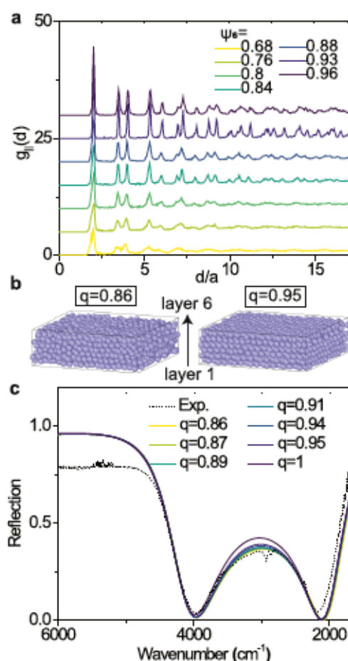
Figure 2. Simulated disordered NC assemblies and their spectra in the Salisbury screen configuration. (a) In-plane pair distribution function ( g_{ij}(d) ) for NC monolayers with various values of the hexatic order parameter ( \psi_6 ). (b) Two example configurations of six layers of disordered NCs with different relative Steinhardt bond-orientational order parameters ( q ). (c) Simulated reflection spectra as a function of q for six layers of 25 nm ITO NCs in a Salisbury screen configuration consisting of 160 nm Ge and 100 nm Au. The dashed line shows the experimental spectrum of a six-layer assembly of 25 nm of 2.7% Sn ITO NCs in the Salisbury screen configuration.
