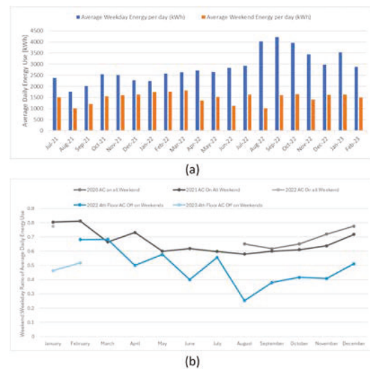
FIGURE 11. Weekday and weekend energy consumption (a) and weekend to weekday energy consumption ratio (b).
