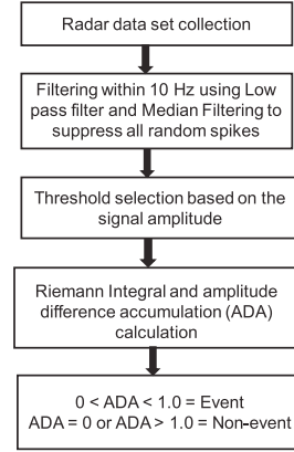
FIGURE 4. Flow chart for algorithm used for occupant presence determination.
