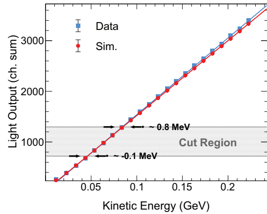
Figure 6. Comparison between data and simulation for calorimeter light output vs. average incident beam electron energy.
