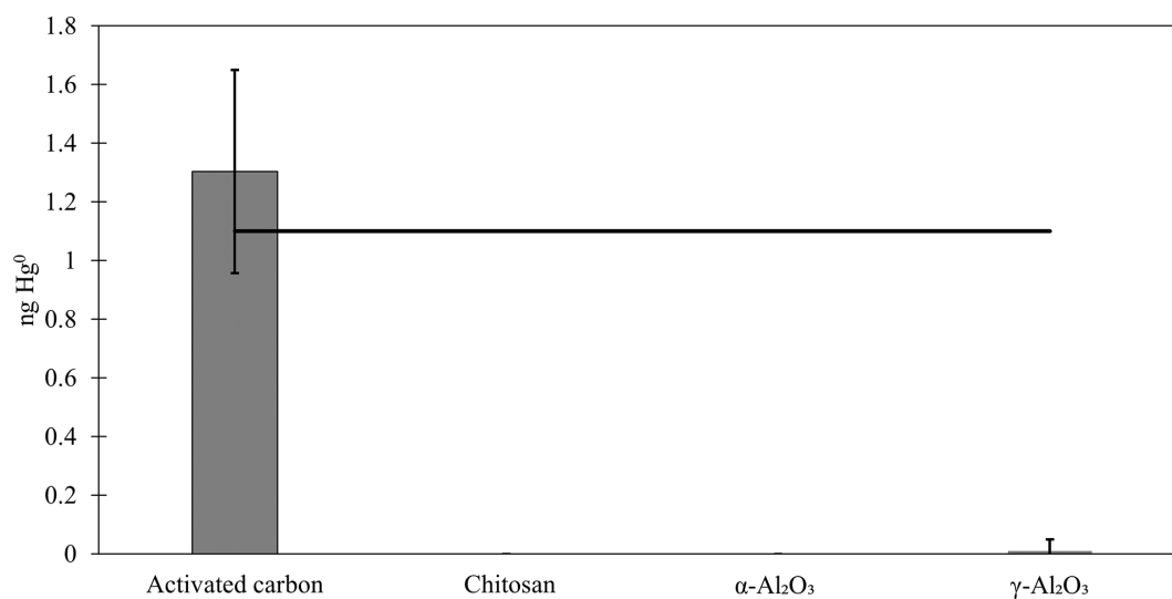
Figure F1. Recovery of \text{Hg}^0 from activated carbon and candidate materials loaded in ambient air by syringe injection. The black line indicates the calculated mass (1.1 \text{ng Hg}^0 ) loaded based on the Dumarey equation.
