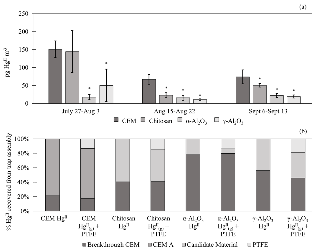
Figure 2. (a) \text{Hg}^{\text{II}} recovery from PTFE + candidate materials deployed in the field for three 1-week campaigns. \text{Hg}^{\text{II}} recovery from traps with first-in-line PTFE membranes ( \text{Hg}^{\text{II}}_{(\text{g})} + \text{Hg}^{\text{II}}_{(\text{p})} ) was combined with traps without PTFE ( \text{Hg}^{\text{II}}_{(\text{g})} ) for statistical analysis ( n = 6 per campaign). Data do not include \text{Hg}^{\text{II}}_{(\text{g})} recovered on breakthrough CEMs. Error bars are \pm 1 standard deviation from the mean. Asterisks (*) indicate a statistically different recovery of \text{Hg}^{\text{II}}_{(\text{g})} on candidate materials compared to CEMs (ANOVA, \alpha \leq 0.05 ). (b) The percent of \text{Hg}^{\text{II}} recovered from each portion of the trap assembly, including from the PTFE, candidate material, first-in-line CEM (CEM A), and/or breakthrough CEM. \text{Hg}^{\text{II}} traps with no upstream PTFE are shown separately from \text{Hg}^{\text{II}}_{(\text{g})} + PTFE traps.
