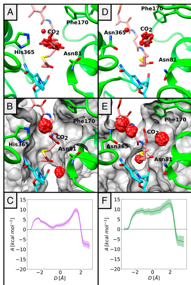
Fig. 3. Left and Right columns represent the E171A and H365 N variants, respectively. (A and D). Active site of KsCcr variants before the nucleophilic attack of the enolate onto CO 2 . The CoA-ester is shown in salmon and NADP + in cyan. Different orientations of carbon dioxide in the simulations represent the tumbling motion of the molecule before product formation. (B and E) Hydration sites located within 5 Å of the C α obtained with SSTMap. (C and F) Minimum free-energy paths from the C2-ene adduct through the enolate to the products (2S)-ethylmalonyl-CoA and NADP + . Parameter D represents the distance between C α and C 2 minus the distance between C α and CO 2 .
