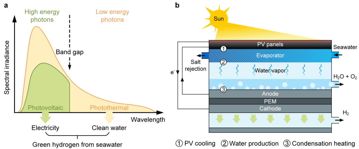
Fig. 1 Solar-powered green hydrogen production from seawater. (a) Full-spectrum utilization enabling in situ water purification and uncompromised electricity production. High-energy photons above the band gap of photovoltaic (PV) panels are converted to electricity (green shadow), whereas waste heat produced by the PV panel due to photothermal (PT) effect (yellow shadow) is used to purify seawater through interfacial thermal distillation. Electricity produced by the PV panel is used to power hydrogen production with PT distilled water fed into the electrolyzer. (b) Schematic of the hybrid solar distillation-water electrolysis (HSD-WE) device. Interfacial thermal evaporator is integrated on the backside of the PV panel to enable PV cooling and in situ water purification. A unidirectional flow driven by the siphon effect is introduced into the evaporator to avoid salt accumulation. The evaporator and electrolyzer are separated by an air gap, which avoids the direct contact between seawater and electrocatalysts. Distilled vapor directly
