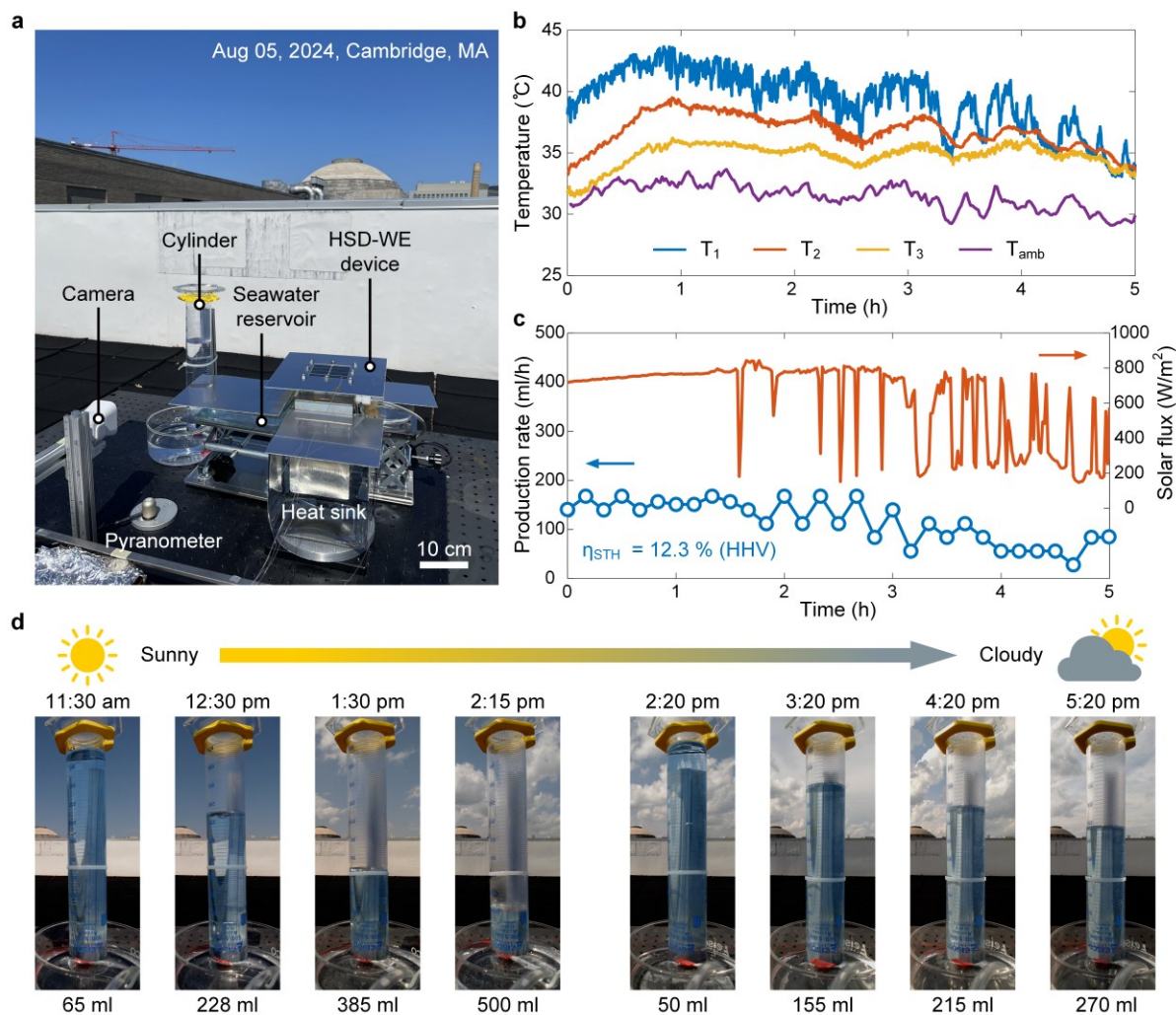
Fig. 5 Outdoor test of the HSD-WE device on a partly sunny day. (a) Image of the experimental setup placed on the rooftop. The outdoor test was performed on a partly sunny day in Cambridge, MA (Aug 05, 2024). (b) Temperature of the HSD-WE device as a function of time during the outdoor test. (c) Solar flux (red curve) and green hydrogen production rate (blue curve) as a function of time. Hydrogen production rate was determined from the water displacement approach. The average HHV-based STH efficiency of the HSD-WE device during the outdoor test was 12.3%. (d) Time-lapse images of continuous green hydrogen production from the HSD-WE device during the outdoor test.
