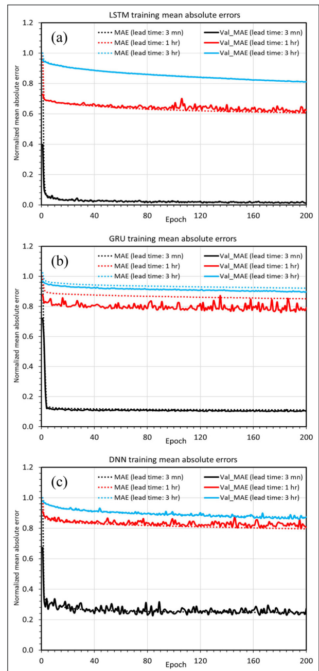
Figure 1 ML accuracy metric based on the mean absolute error (dotted lines) during the training process as a function of iterations (epochs) for three different ML models a) LSTM, b) GRU, and c) DNN at forecast lead times of \tau = 3 minutes (black), 1 hour (red), and 3 hours (blue). All absolute errors are normalized by the errors at the first iteration (epoch 1) for better comparison among different lead times. Solid lines denote the mean absolute errors for the corresponding validation dataset in each training process, and the recurrent timesteps M = 5 .
