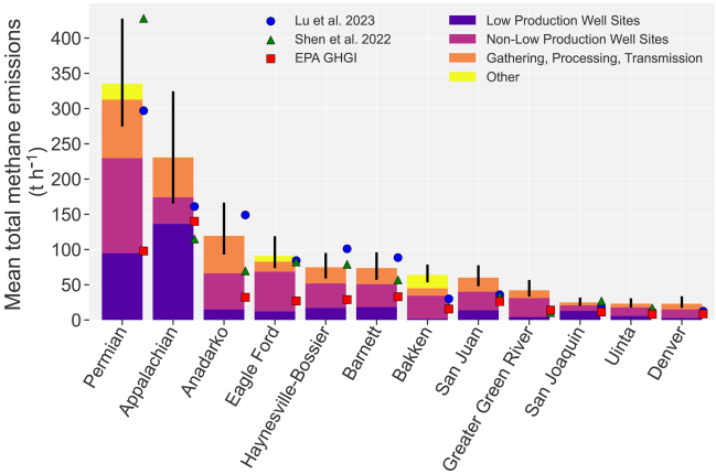
Figure 5. Basin-level differences in modeled mean total methane emissions and comparison with the EPA GHGI (Maasakkers et al., 2023), TROPOMI-derived estimates (Shen et al., 2022), and GOSAT-derived estimates (Lu et al., 2023). See Fig. S11 for a similar chart showing the state-by-state breakdown for the top 10 emitting US states based on the EI-ME inventory estimates.
