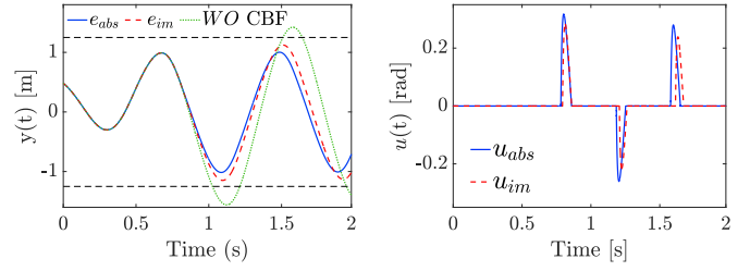
Fig. 2: Lateral displacement from center trajectories y(t) (left) and trajectories of CBF intervention u(t) (right) given by \Delta u(t) \triangleq u(t) - k(x(t), t) , where k(x(t), t) is the nominal controller. The black dotted lines in (left) are \pm y_{max} , and the T_p and T_i are 0.3 and 0.175 s, respectively (subscripts abs: Abstraction, im: Immersion).
