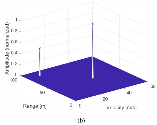
Fig. 9. 2-D boosted CS on sparse data. (a) Initial pairing. (b) After amplitude dealiasing. The red \times denotes the actual positions of the targets.
