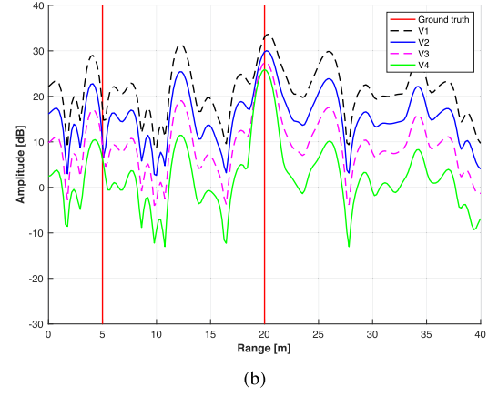
Fig. 17. Range profiles of victim radars at various distances without interference mitigation in (a) conventional chirp and (b) nested co-chirp transmission.
