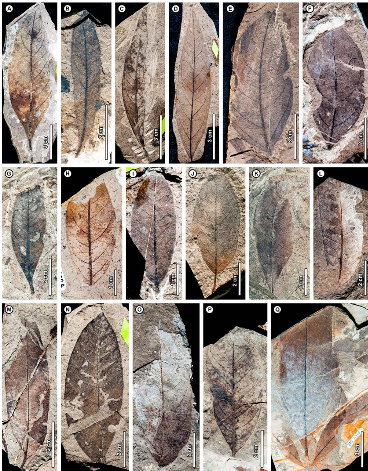
FIGURE 10. Exemplars of morphotypes GZ084–GZ112, entire leaves. A, GZ096, “ Nectandra ” prolifera , USNM PAL 40429b; B, GZ097, “ Nectandra ” prolifera , USNM PAL 40471e; C, GZ098, “ Nectandra ” prolifera , USNM PAL 40471d; D, GZ099, “ Nectandra ” prolifera , USNM PAL 40471f; E, GZ100, BAR 4685; F, GZ101, (BAR) RP3_2005_501; G, GZ102, (BAR) RP3_2005_869; H, GZ103, BAR 4500; I, GZ104, “ Dalbergia ” patagonica ; USNM 40416a; J, GZ105, BAR 4308; K, GZ106, (BAR) RP3_2005_905; L, GZ107, (BAR) RP3_2005_1019; M, GZ108, BAR 4677; N, GZ109, “ Inga ” patagonica , USNM PAL 40402; O, GZ110, (BAR) RP3_2005_506; P, GZ111, (BAR) RP3_2005_731; Q, GZ112, BAR 4310.
