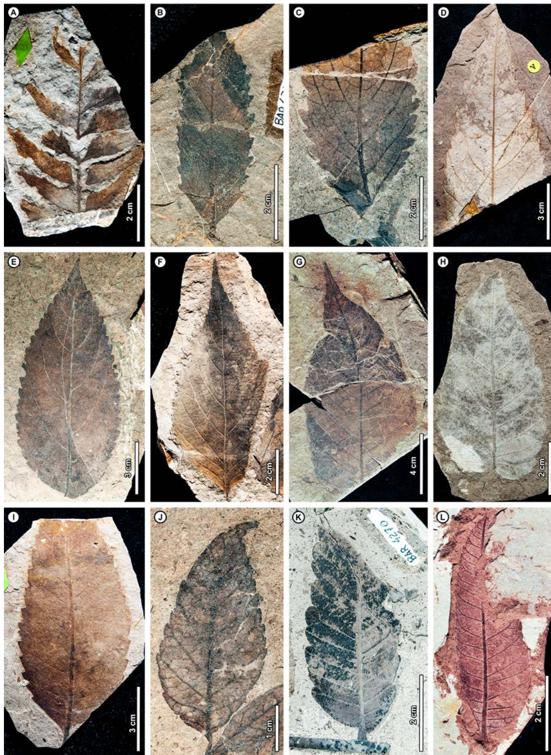
FIGURE 6. Exemplars of morphotypes GZ036–GZ047, toothed leaves. A, GZ036, Lomatia preferruginea , USNM PAL 219145; B, GZ037, BAR 4272; C, GZ038, (BAR) RP3_2005_1105; D, GZ039, "Banara" cuadrae , USNM PAL 40450c; E, GZ40, BAR 4662; F, GZ041, "Celtis" ameghinoi , USNM PAL 40395a; G, GZ042, (BAR) RP3_2005_874; H, GZ043, "Eucryphia" tertiaria , USNM PAL 40456; I, GZ044, "Tabebuia" ipiformis , USNM PAL 40508b; J, GZ045, (BAR) RP3_2005_827; K, GZ046, "Cupania" grosse-serrata , BAR 4270; L, GZ047, Anacardites pichileufensis , (BAR) RP3_2005_812.
