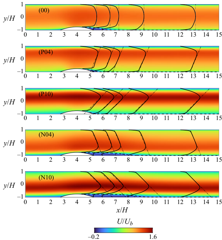
Figure 6. Mean streamwise velocity contours. — indicates mean streamwise velocity profiles at x/H = 4, 5.5, 6, 8, \text{ and } 12 ; --- indicates separating streamlines; - · - indicates velocity gradient ( \partial U/\partial y ) corresponding to 2\Omega . From top to bottom: Ro_b = 0, 0.42, 1.0, -0.42, -1.0 .
