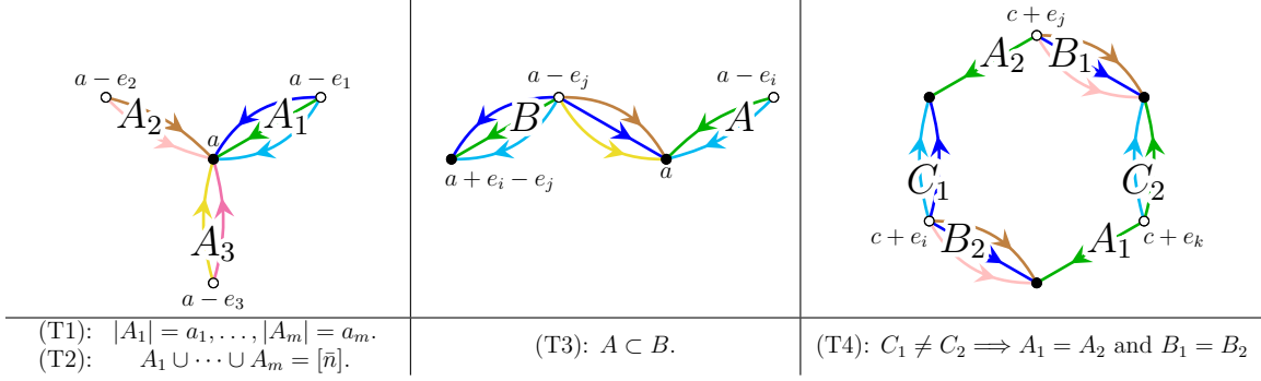
FIGURE 2. Axioms for trianguloids.
