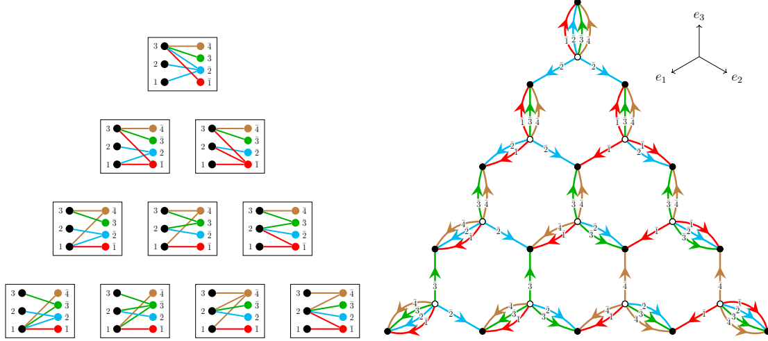
FIGURE 1. A family \mathcal{T}(\tau) of trees for a triangulation \tau of Q_{K_{m,n}} for m=3, n=4 (left), and the corresponding trianguloid \mathbb{T} := \mathbb{T}_\tau (right). The white (resp., black) vertices of \mathbb{T} are the lattice points of P_G^- = (n-1)\Delta_{[m]} (resp., of P_G = n\Delta_{[m]} ). Each point b \in P_G^- corresponds to a tree T_{\mathbb{T}}(b) \in \mathcal{T}(\tau) with \text{LD}^-(T_{\mathbb{T}}(b)) = b so that the outgoing arrows of b in \mathbb{T} in the direction of e_i are labeled by the neighbors of i in T_{\mathbb{T}}(b) .
