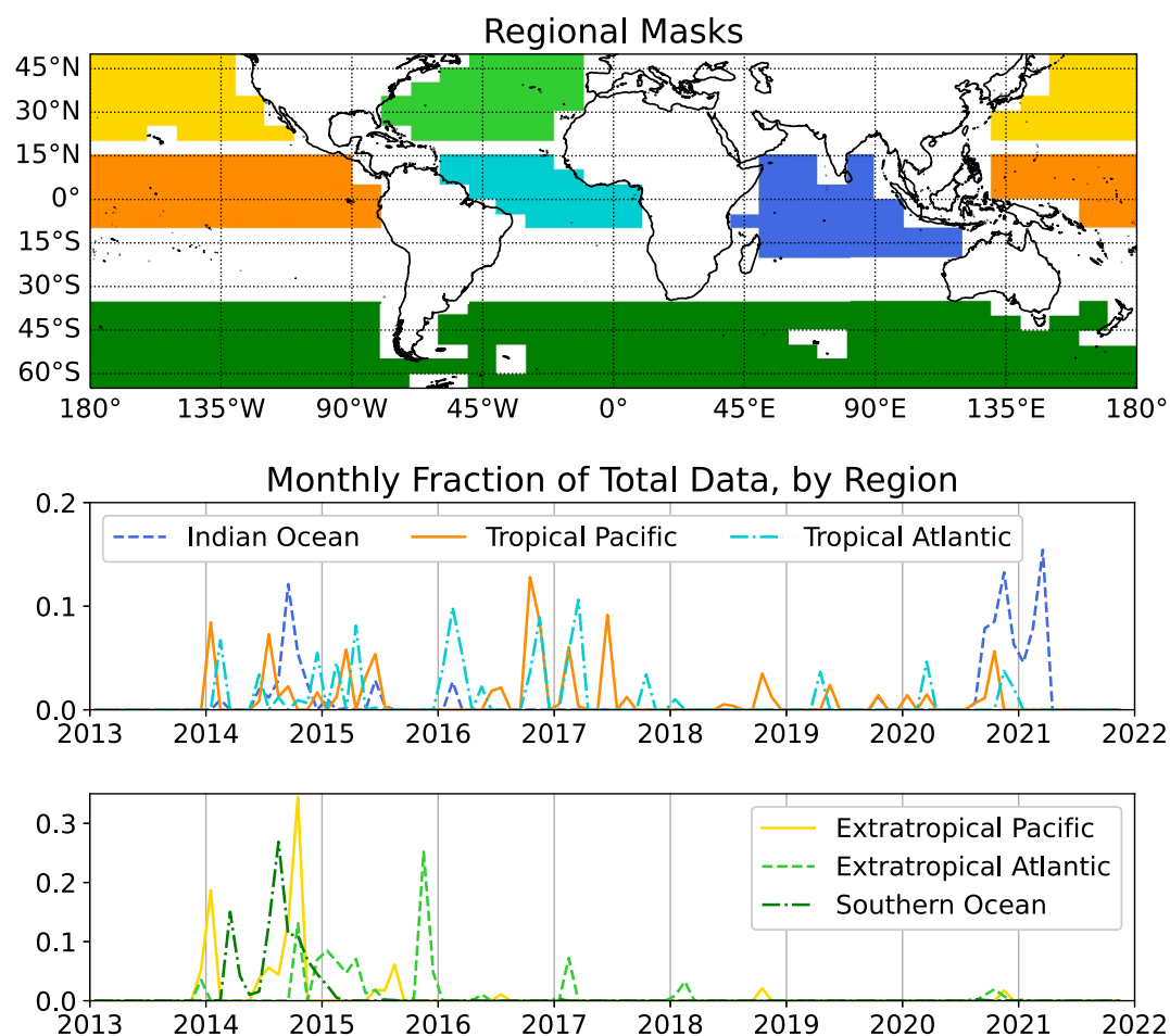
Figure 3. Regional data masks. Top: data collected inside each colored region are assigned to that region. Middle, bottom: the monthly fraction of the total data collected in each region.
