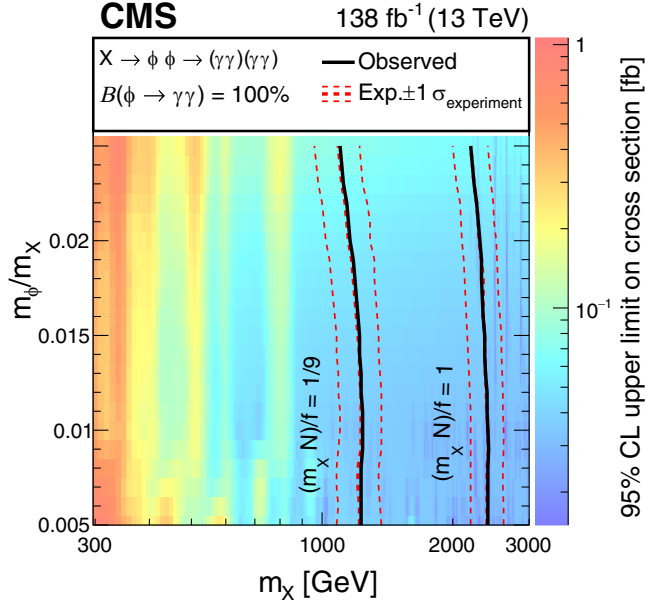
FIG. 3. Exclusion limits at 95% CL on \sigma[X \rightarrow \phi\phi \rightarrow (\gamma\gamma)(\gamma\gamma)] displayed in the (m_\phi/m_X) - m_X plane. Branching fractions ( \mathcal{B} ) of both X \rightarrow \phi\phi and \phi \rightarrow \gamma\gamma are assumed to be 100%. The black (red) lines represent the observed (expected) mass exclusions corresponding to different assumptions of (m_X N)/f . The observed upper limits on the cross section are shown on the color z axis.
