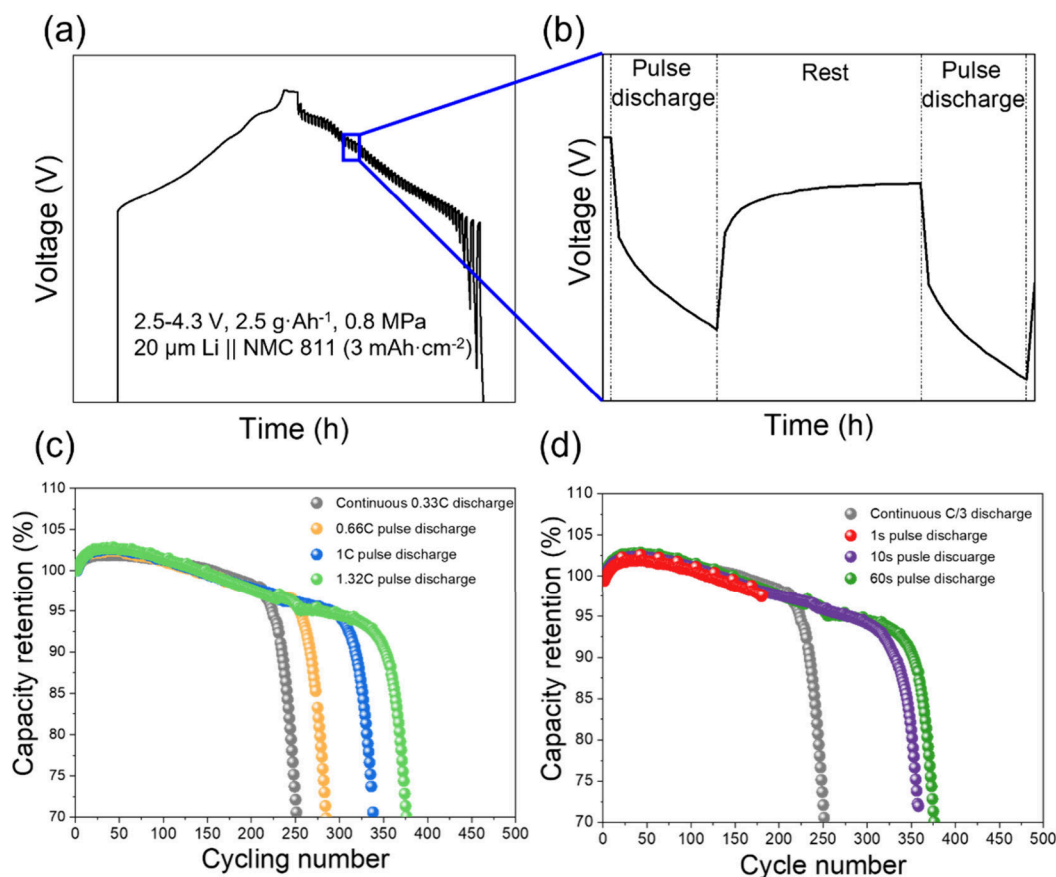
Figure 7. Pulse discharge protocol and cycling performance of 20 \mu\text{m} Li||NMC 811 ( 3 \text{ mAh}\cdot\text{cm}^{-2} ) pouch cell (2.5–4.3 V) with electrolyte amount of 2.5 \text{ g}\cdot\text{Ah}^{-1} and 0.8 MPa external pressure: (a, b) voltage curve of pulse discharge, (c) capacity retention with different pulse discharge currents, and (d) capacity retention with different pulse discharge time.
