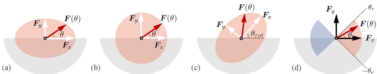
Fig. 2 Illustration of the different load types that may be specified by the general loading definition; a the elliptical domain when \|\mathbf{F}_x\| \neq \|\mathbf{F}_y\| ; b the particular case when \|\mathbf{F}_x\| = \|\mathbf{F}_y\| for the circular domain; c the rotated elliptical domain; d the constrained load domain
