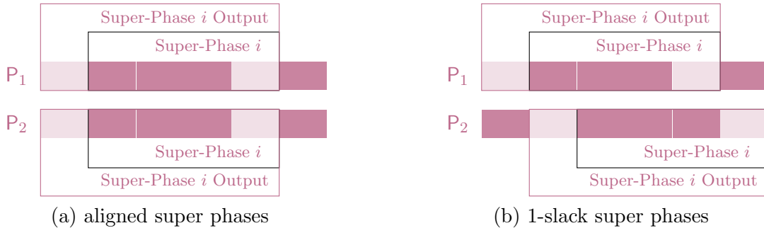
Figure 3: Illustration of the super-phase expansion and how parties extract the super-phase output. represents the phase where a party mines input messages with her output suggestion, and is the dummy phase. The i -th super phase is represented by ; and the associated phases to extract output are depicted with .
