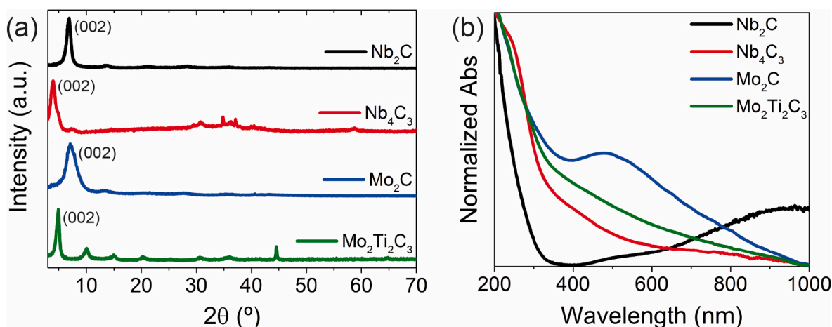
Fig. 2. (a) XRD patterns and (b) UV-vis spectra of Nb 2 C, Nb 4 C 3 , Mo 2 C and Mo 2 Ti 2 C 3 MXenes.
