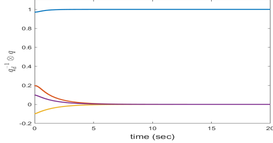
Fig. 6. Time response of \tilde{q}
