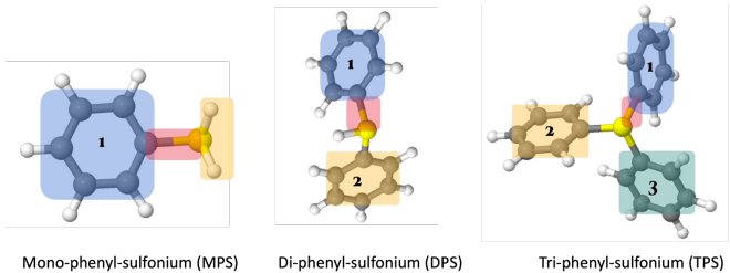
FIG. 1. Mono-, Di-, and Triphenylsulfonium systems with their fragmentations. The gray spheres are carbon atoms, the yellow sphere is a sulfur atom, and the white spheres are hydrogen atoms. The translucent blue, red, yellow and green boxes indicate the atoms associated with the three or four LASSCF fragments.
