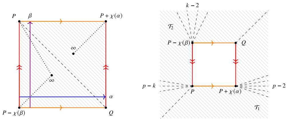
Figure 19. The quadrilateral \mathcal{Q} from two different perspectives. On the left-hand side, we can see the curves \alpha and \beta . Any dotted line represents a ray from a vertex of \mathcal{Q} to a point at infinity. These rays are better represented on the right-hand side.
