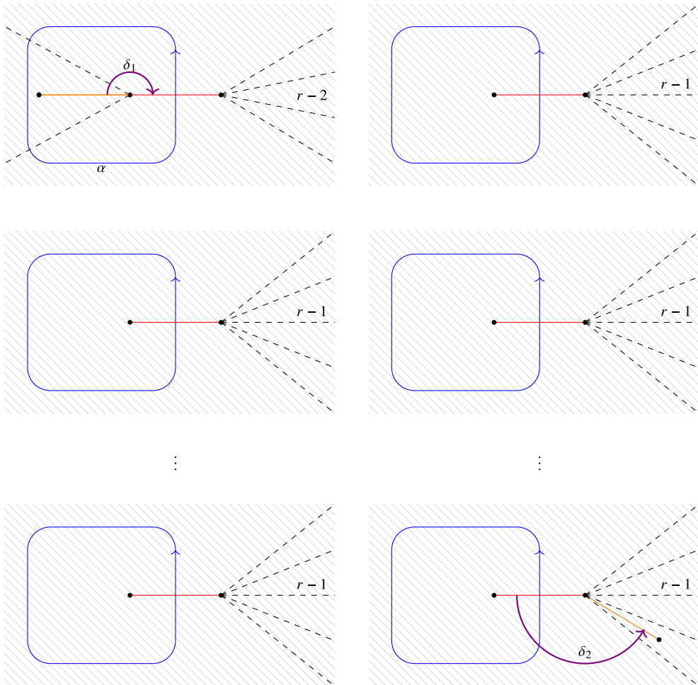
Figure 42. Realization of the trivial representation in the stratum \mathcal{H}_1(n+1, nr-n-1; -r^n) . This figure depicts the extreme case in which m_1 = n+1 , that is, a_1 = 2 , a_2 = \dots = a_n = 1 and b_1 = r-2 and b_2 = \dots = b_n = r-1 . The close curve \alpha has index n+1 whereas the close \beta has index 0. In this case, n = kr - 1 for some k \in \mathbb{Z}^+ .
