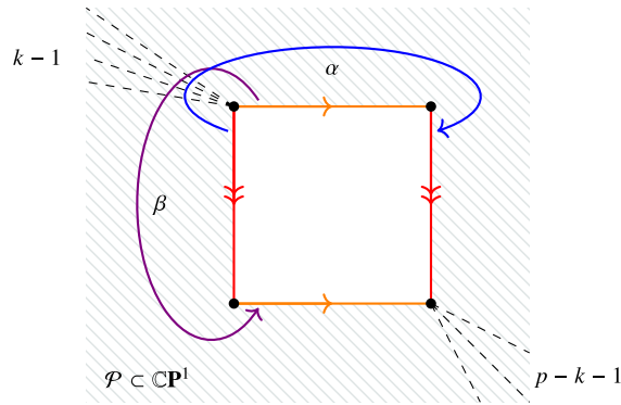
Figure 18. Realizing a genus-one translation surface with one single pole of order p , nonpositive volume and rotation number equal to \gcd(k, p) .
