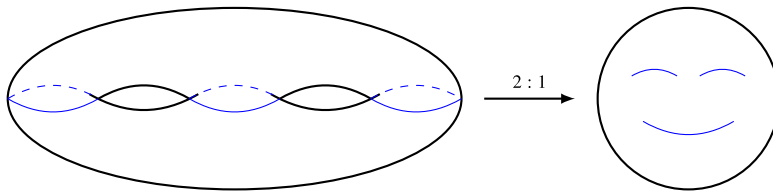
Figure 1. A 2-fold branched covering \pi : X \longrightarrow \mathbb{CP}^1 .
