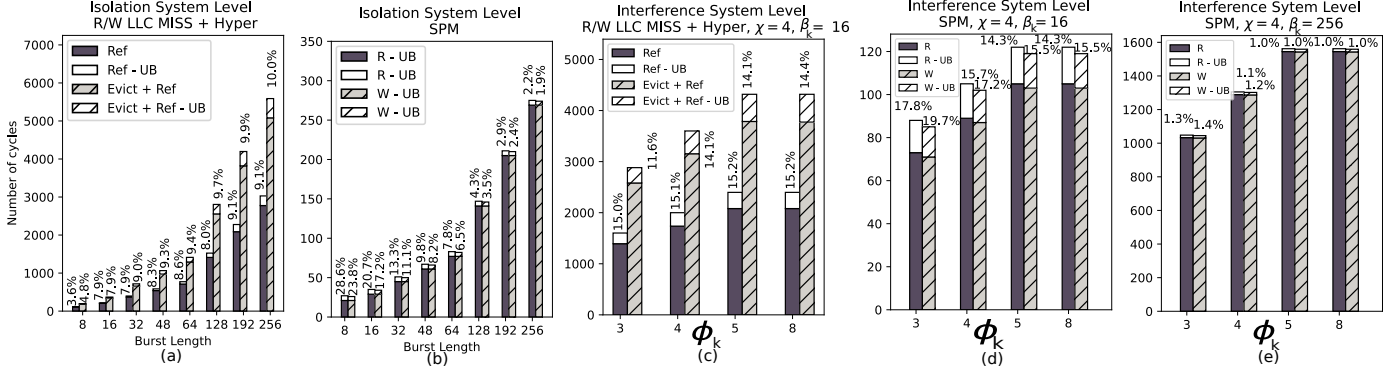
Fig. 10: Services times under interference.
