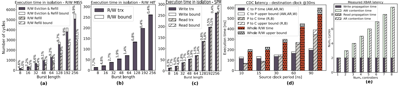
Fig. 9: Services time in isolation.
