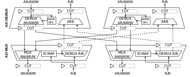
Fig. 8: AXI Crossbar block diagram
