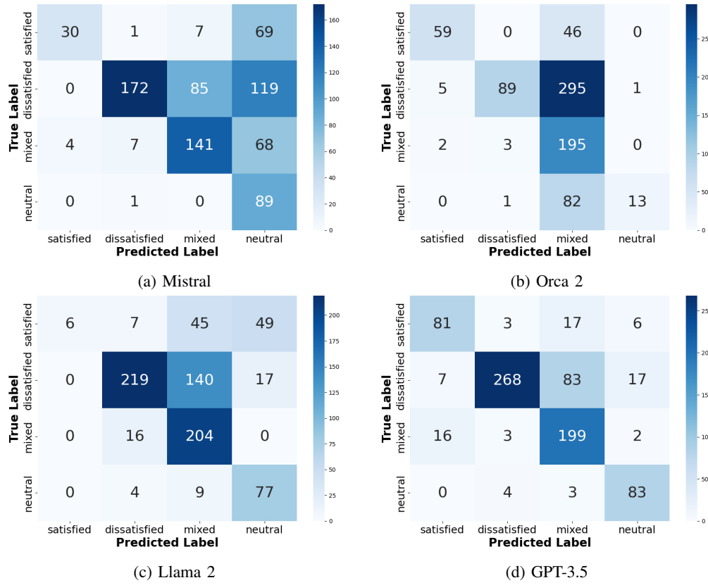
Fig. 2: Confusion metrics for the four LLMs on the entire SMILE-College dataset .
