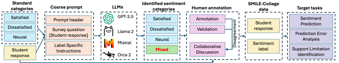
Fig. 1: Overall framework for sentiment annotation with human-machine collaboration.
