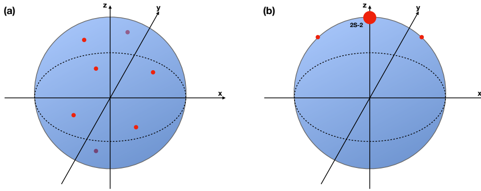
Figure 3: (a) A spin- S state can be represented as 2S points on a Bloch sphere, where the SO(3) rotation can be viewed as a rigid body rotation of the 2S points, here S = 7/2 . (b) An example of a spin- S state which breaks SO(3) symmetry to \mathbb{Z}_2 , generated by the \pi rotation with respect to S_z .
