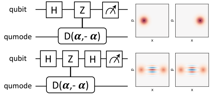
Fig. 3. Bosonic Qiskit circuit and Wigner functions showing the stages of preparation of a non-deterministic cat state. In the upper panel, the qumode is projected onto either the |+\alpha\rangle or |-\alpha\rangle coherent state, depending on the outcome of the qubit measurement ( |0\rangle or |1\rangle ) following the controlled displacement. In the lower panel, the qubit is first transformed using a Hadamard gate prior to measurement, and the qumode is thus projected onto an even ( |0\rangle ) or odd ( |1\rangle ) cat state upon measurement of the ancilla. These two outcomes can be differentiated by the color of the fringes.
