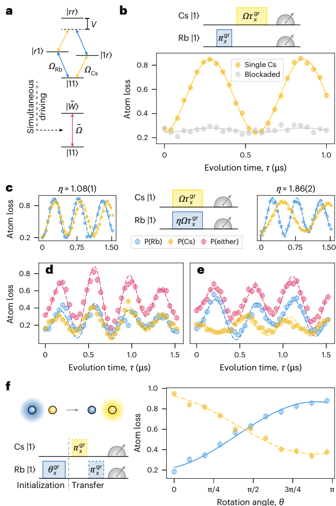
Fig. 3 | Dual-species Rydberg blockade and dynamics. a , Simplified Rb–Cs gr manifold level diagram depicting the doubly excited state shifts out of resonance due to the Rydberg blockade. Under simultaneous driving, the ground state couples to a singly excited W -like state |\tilde{W}\rangle , with enhanced Rabi frequency \tilde{\Omega} (Supplementary Information Section 13). b , Rb atoms were prepared in |r\rangle , followed by Rabi driving of the Cs atoms. Conditioning on single versus pair loading and the correct preparation of the Rb atom (Supplementary Information Section 9), the fitted Cs oscillation amplitude was strongly suppressed from A = 0.606(18) to A = 0.036(24) . \pi_x denotes a \pi pulse around the x -axis. c , In the absence of the other species, Rb and Cs exhibit typical Rydberg Rabi oscillations. d, e , Observed and simulated Rydberg dynamics under simultaneous driving. d , The Rabi frequencies are balanced such that \eta = \Omega_{\text{Rb}}/\Omega_{\text{Cs}} = 1.92(1)/1.78(1) = 1.08(1) . e , The Rabi frequencies are unbalanced such that \eta = 1.93(1)/1.04(1) = 1.86(2) . When paired, enhanced oscillations occur at 2.53(2) MHz ( d ) and 2.17(2) MHz ( e ), as expected from \tilde{\Omega} . The relative excitation probability is theoretically given by \Omega_i^2/\tilde{\Omega}^2 , i \in \{\text{Rb}, \text{Cs}\} . These observations are affected by SPAM errors but are described well by numerical simulations that taking these into account (dashed lines in c–e ). f , For the interspecies quantum state transfer, the Rb atom is initialized in an arbitrary state through R_x(\theta) (solid blue line). After initialization, a \pi pulse on Cs generates \langle ZZ \rangle correlations, and a subsequent \pi pulse on Rb disentangles the atoms and completes the transfer (dashed yellow line).
