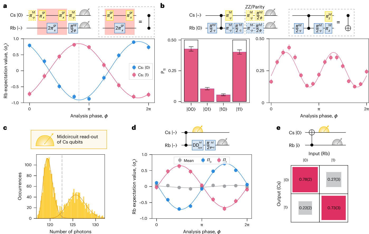
Fig. 4 | Entanglement of long-lived hf qubits and midcircuit QND read-out.
