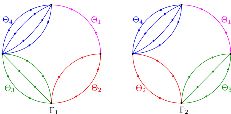
Fig. 1 An example of a permuted pair. Note that \Gamma_1 and \Gamma_2 both consist of \Theta_i (where 1 \leq i \leq 4 ) glued along essential vertices
