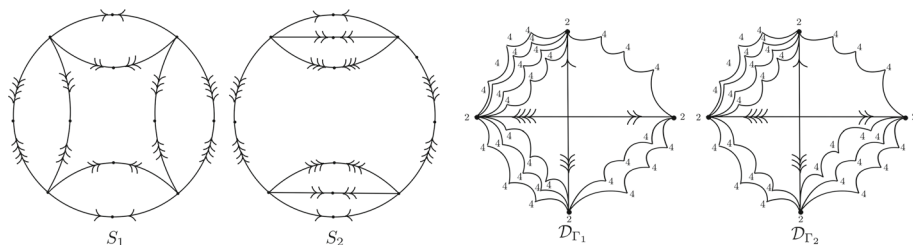
Fig. 6 Here, the defining graphs \Gamma_1 and \Gamma_2 are the permuted pair from Fig. 1, so they satisfy the conditions of Lemma 2. The singular sets S_i of X_i , which are four-sheeted covers of \mathcal{D}_{\Gamma_i} for i = 1, 2 are shown on the left. Note that X_1 and X_2 are homotopic but not homeomorphic
