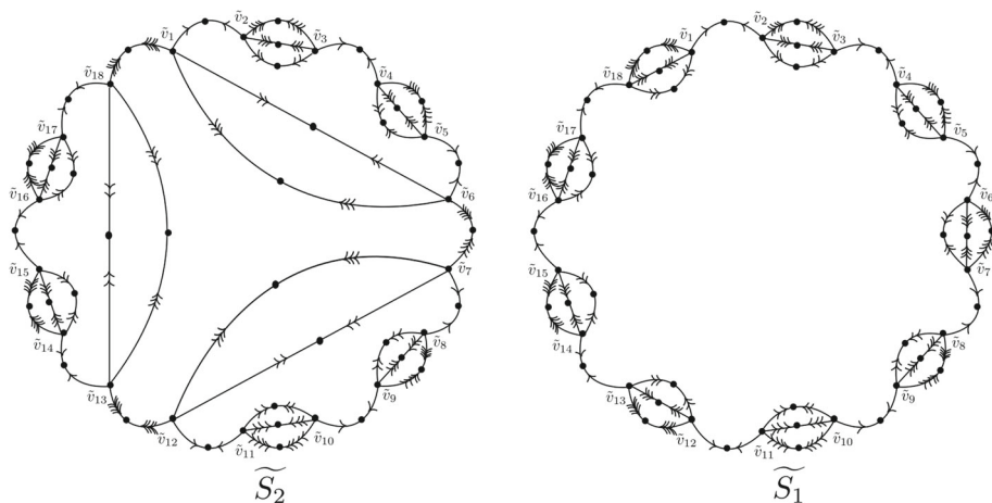
Fig. 5 Two homotopic but non-homeomorphic covers of the singular set of W_\Gamma from Fig. 2. Instead of labeling the edges with numbers, we use different numbers of arrows
