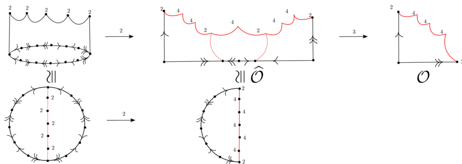
Fig. 3 A tower of covers illustrating the lemma. Here, D^2(2, 2, 2, 2, 2, 2) is a six-fold cover of an orbifold with four reflection edges
