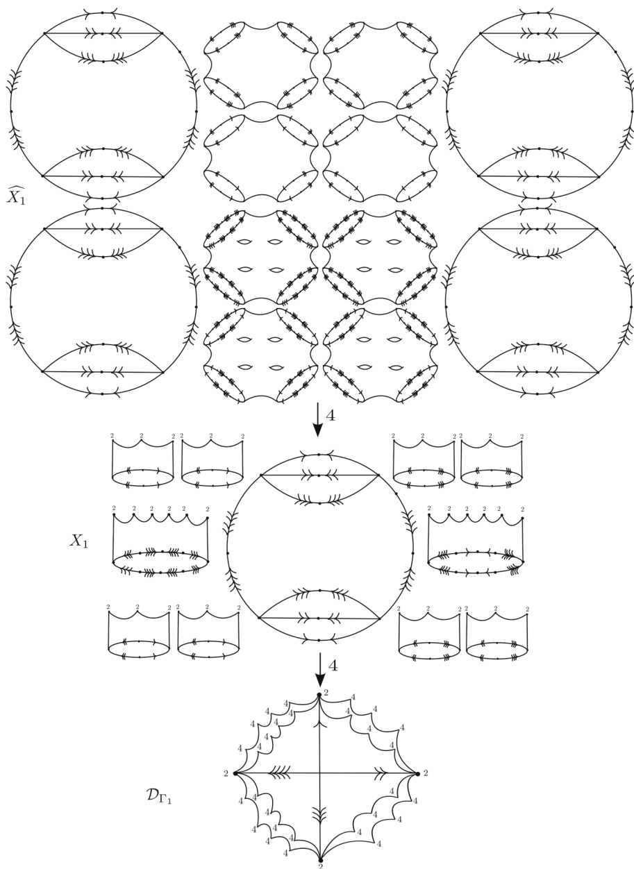
Fig. 8 A tower of covers constructed in the proof of Lemma 3. Note that \widehat{X}_1 is homotopic to a hyperbolic P-manifold
