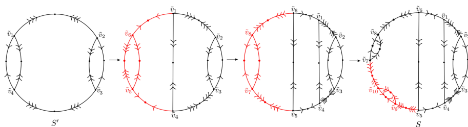
Fig. 10 Construction of a S \in \mathcal{S} from a cycle of generalized \Theta graphs. The edges and vertices added at each step are depicted in red
