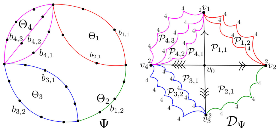
Fig. 2 A cycle of generalized \Theta graphs \Psi along with its Davis orbicomplex \mathcal{D}_\Psi . We label edges e_l in the singular star S with l arrows. Note that each branch b_{i,j} \in \Psi determines an orbifold \mathcal{P}_{i,j} \in \mathcal{D}_\Psi
