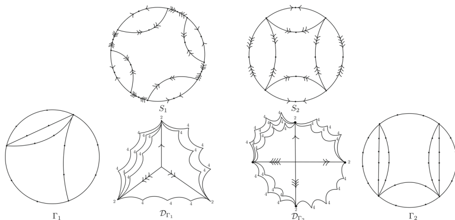
Fig. 7 S_1 and S_2 are non-homeomorphic singular sets of homotopic eight- and four-sheeted covers of \mathcal{D}_{\Gamma_1} and \mathcal{D}_{\Gamma_2} . Thus, neither \Gamma_1 nor \Gamma_2 is repetitive and \Gamma_1 and \Gamma_2 do not form a permuted pair, yet any set \mathcal{X}'' that contains all finite-sheeted covers of \mathcal{D}_{\Gamma_1} and \mathcal{D}_{\Gamma_2} is not topologically rigid
