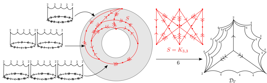
Fig. 9 An example of a finite-sheeted cover of a Davis orbicomplex \mathcal{D}_\Gamma that does not satisfy Assumption 1. The singular set S is not necessarily planar; in this example, S (depicted in red) embeds on a torus
