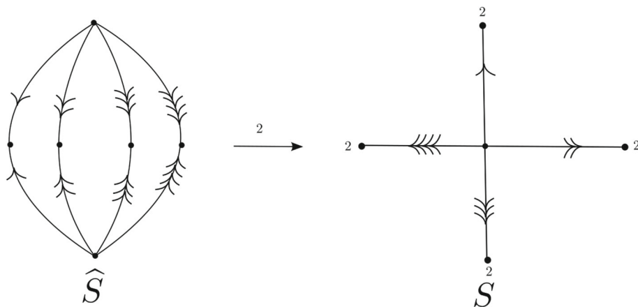
Fig. 4 A generalized \Theta graph with four branches two-fold covers the singular subset of the orbifold from Fig. 2. Here, N = 4
