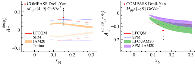
FIG. 2. Left panel: Measured average Siverts TSA and theoretical predictions from different models from Ref. [52]. The dark-shaded (light-shaded) predictions are evaluated with (without) the sign-change hypothesis. Right panel: Measured average transversity TSA and theoretical predictions from different models from Ref. [52]. Otherwise as in Fig. 1.
