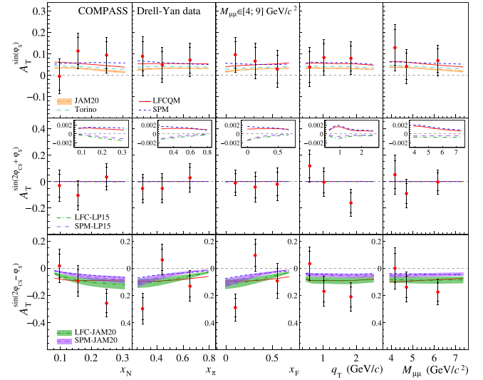
FIG. 1. Kinematic dependences of the Sivers, pretzelosity, and transversity TSAs (top to bottom). Inner (outer) error bars represent statistical (total experimental) uncertainties. For theoretical predictions see text.
