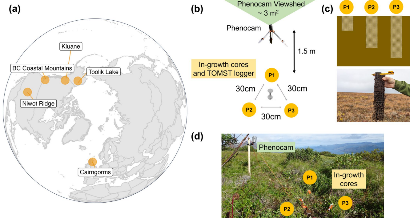
FIGURE 1 | Our study included five sites, each with between 5 and 12 plots which contained paired phenocams and in-growth cores. (a) Polar projection map of the five Arctic, subarctic and alpine tundra sites included in this study. Map lines delineate study areas and do not necessarily depict accepted national boundaries. (b) Birds-eye-view schematic of the subplots, showing the location of in-growth cores P1, P2 and P3 in relation to the phenocam and the TOMST microclimate logger. (c) Cross-section schematic of the differential in-growth core depths in the soil profile at sites with permafrost (sites without a shallow thaw depth in the first half of the season and permafrost had the same depth for all cores). Photograph of a P3 core removed from Toolik in 2022 (Image Credit: Ruby An). (d) Photograph of Kluane Subplot 8 with a phenocam pointed northwards, alongside three buried in-growth cores in summer 2021 (Image Credit: Madelaine Anderson).
