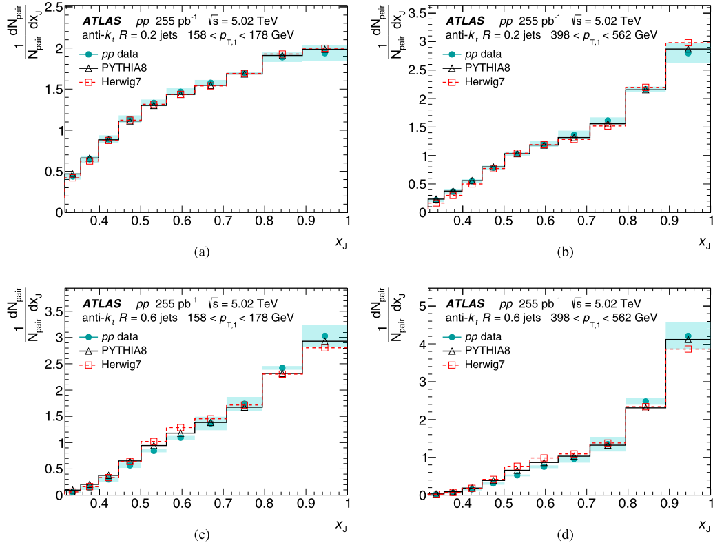
FIG. 11. The dijet-yield-normalized x_J distributions in pp collisions, and in PYTHIA 8 and HERWIG7 simulations, for (a), (b) R = 0.2 and (c), (d) R = 0.6 jets with (a), (c) 158 < p_{T,1} < 178 GeV and (b), (d) 398 < p_{T,1} < 562 GeV. Jets are selected with |y| < 2.1 and |\phi_1 - \phi_2| > 7\pi/8 . The boxes correspond to systematic uncertainties and the bars to statistical uncertainties.
