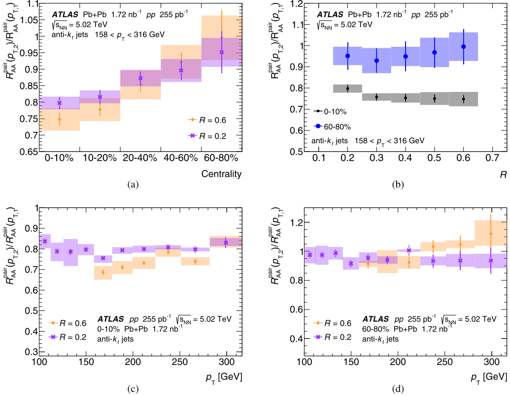
FIG. 7. The double ratio R_{AA}^{pair}(p_{T,2})/R_{AA}^{pair}(p_{T,1}) of the subleading to leading jet R_{AA}^{pair} distributions in dijets as a function of (a) centrality and (b) jet radius for 158 < p_T < 316 GeV, and as a function of jet p_T for (c) 0–10% and (d) 60–80% central Pb+Pb collisions. Jets are selected with |y| < 2.1 and |\phi_1 - \phi_2| > 7\pi/8 . The boxes correspond to systematic uncertainties and the bars to statistical uncertainties.
