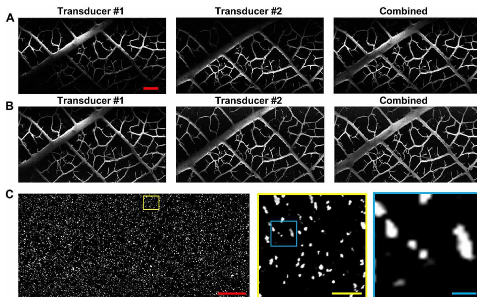
Fig. 2. PUV-PAM of leaf skeleton and carbon particles. (A) PUV-PAM of a leaf skeleton phantom using single transducers and dual transducers without time-dependent gain compensation (TDGC). (B) PUV-PAM of a leaf skeleton phantom using single transducers and dual transducers with TDGC. (C) PUV-PAM images of carbon particles using dual transducers with TDGC. Close-up images are extracted from the rectangle areas in corresponding colors. Red scale bars, 500 \mu\text{m} . Yellow scale bar, 50 \mu\text{m} . Blue scale bar, 10 \mu\text{m} .
