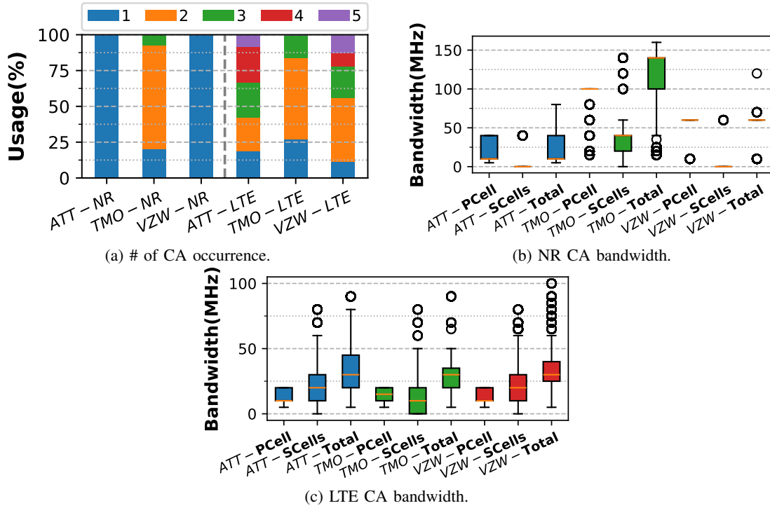
Fig. 8: Number of aggregated DL channels and bandwidth.
