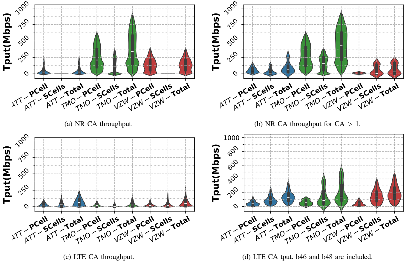
Fig. 9: DL CA throughput performance between operators in NR and LTE
