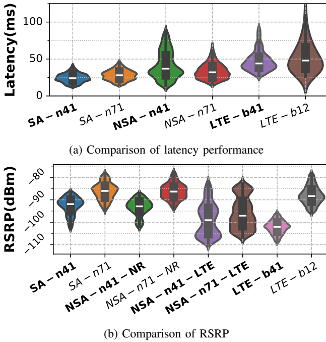
Fig. 13: Comparison of latency performance and RSRP in TMO low-bands (normal) and mid-bands (bolded)
