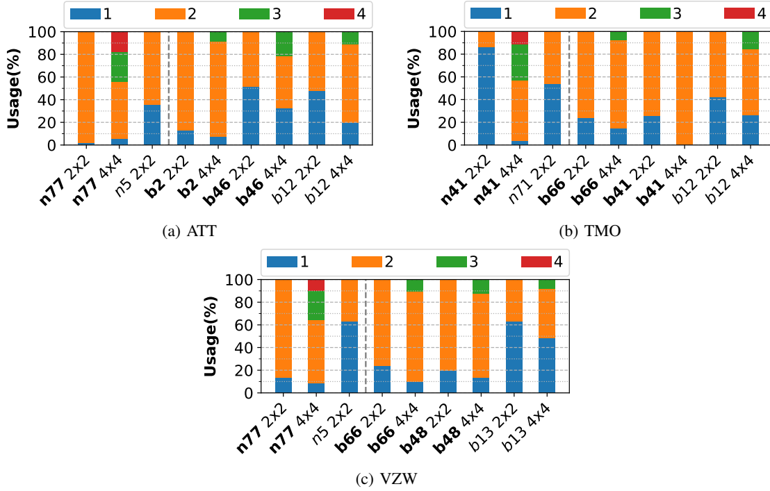
Fig. 12: RI values for the operators and MIMO modes in low-bands (normal) and mid-bands (bolded).
