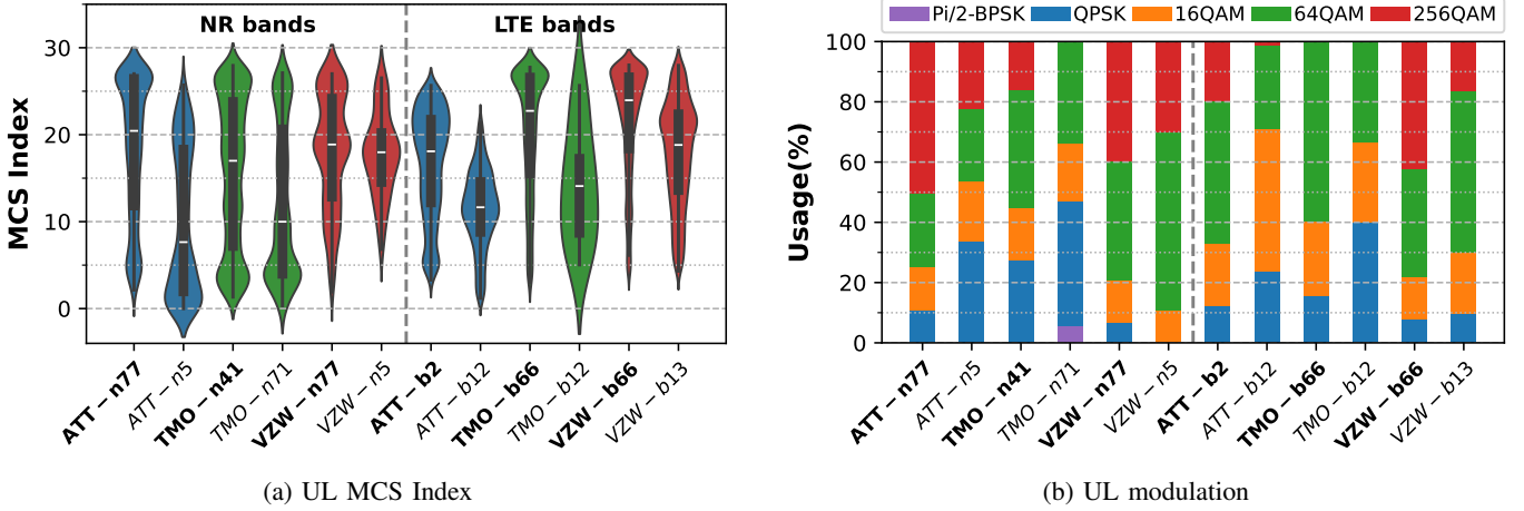
Fig. 11: Comparison of uplink MCS, CQI, TX power, and modulation of NR and LTE in low-bands (normal) and mid-bands (bolded).
