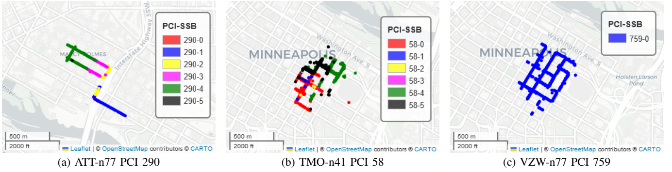
Fig. 4: PCI-SSB index maps of mid-band channels.
