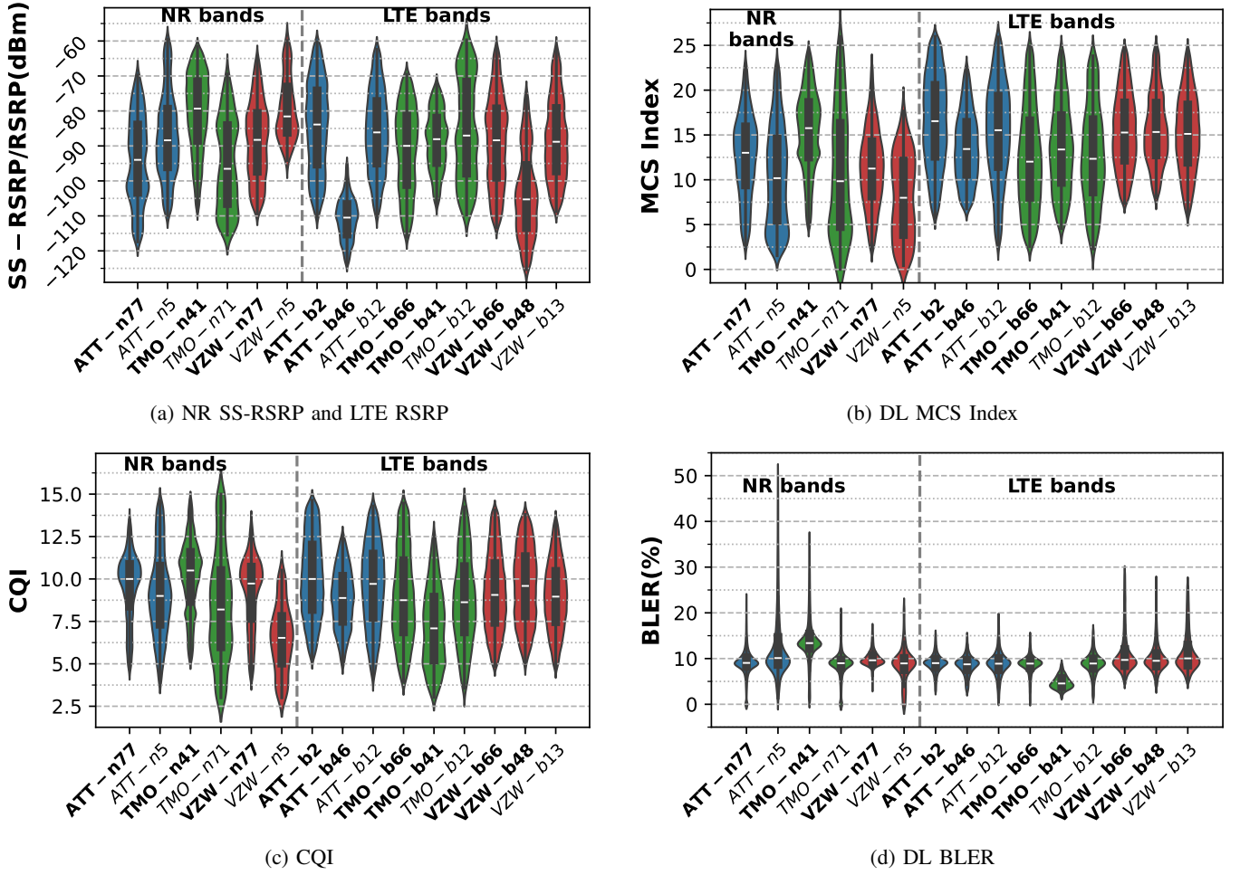
Fig. 6: Comparison of RSRP, DL MCS, CQI, and DL BLER of NR and LTE in low-bands (normal) and mid-bands (bolded).
