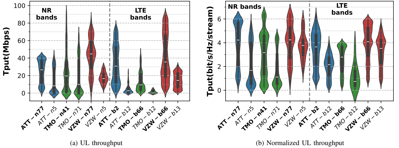
Fig. 10: UL throughput comparison of NR and LTE in low-bands (normal) and mid-bands (bolded)
