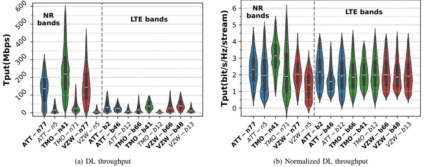
Fig. 5: DL throughput comparison of NR and LTE in low-bands (normal) and mid-bands (bolded)
