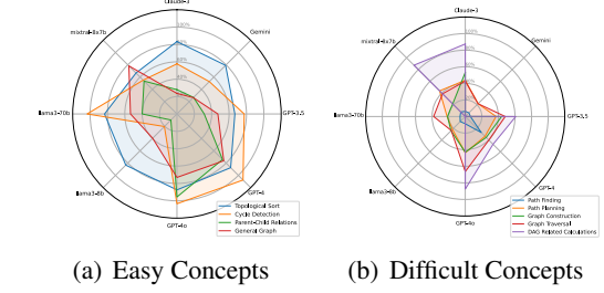
Figure 6: Passing rate of LLMs on graph concepts. Part (a) presents the passing rate on easy concepts, and part (b) presents the passing rate on difficult concepts.
