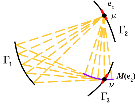
Figure 3: An example of a pairing. Each dashed triangle is a similar copy of \triangle p_1 p_2 p_3 .
