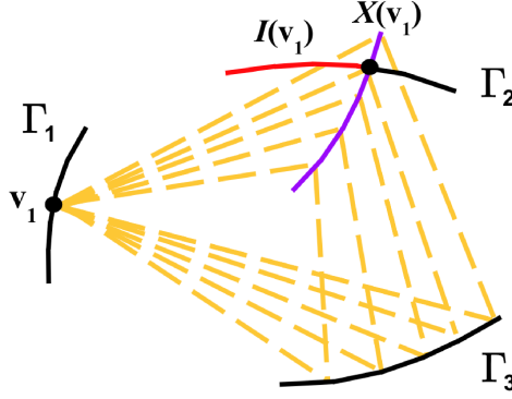
Figure 1: The construction from Lemma 1. Each dashed triangle is a similar copy of \triangle p_1 p_2 p_3 , and the purple arc is f_{v_1}(\Gamma_3) . (We draw \Gamma_2 and \Gamma_3 instead of \overleftrightarrow{\Gamma_2} and \overleftrightarrow{\Gamma_3} for visual clarity.)
