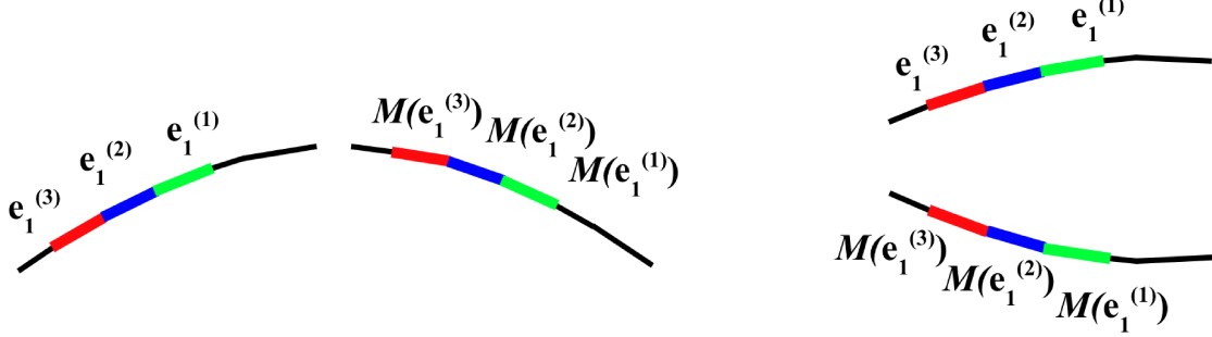
Figure 2: (Left) Monotonically increasing pairing. (Right) Monotonically decreasing pairing.
