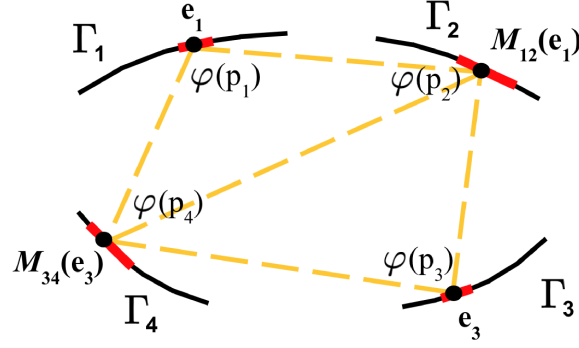
Figure 6: An example quadruple from Case 2 in the proof of Theorem 11. The pairing M_{12} is produced using \triangle p_1 p_2 p_4 and the pairing M_{34} is produced using \triangle p_2 p_3 p_4 .
