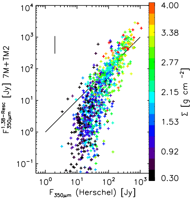
Fig. 6. Total flux within the 4\sigma contours of the 7M+TM2 PBCOR images rescaled to 350\text{ }\mu\text{m} , as a function of the 350\text{ }\mu\text{m} flux from Herschel . For the rescaling of the ALMA 1.38 mm flux to 350\text{ }\mu\text{m} we use optically thin assumptions with \beta = 1.75 and the dust temperature from the Herschel SED fitting. The black line is the identity line, and the color scale is proportional to the clump surface \Sigma , again from Herschel . The vertical black line shows the spread of values that the 350\text{ }\mu\text{m} -rescaled 1.38 mm flux can assume for different dust temperatures and opacities.
