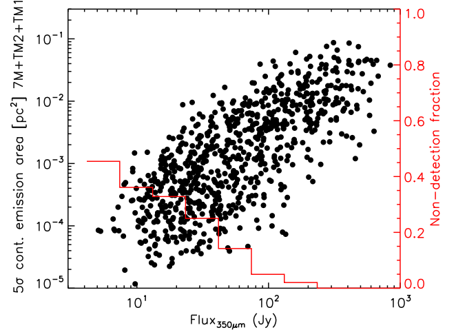
Fig. 7. ALMA 1.38-mm total emission area above 5\sigma in the 7M+TM2+TM1 images as a function of the Hi-GAL 350\text{ }\mu\text{m} flux ( r_p=0.74 ). The red histogram reports the fractional distribution of the 350\text{ }\mu\text{m} flux for ALMAGAL sources with no 5\sigma detection (to be read on the red right y-axis).
