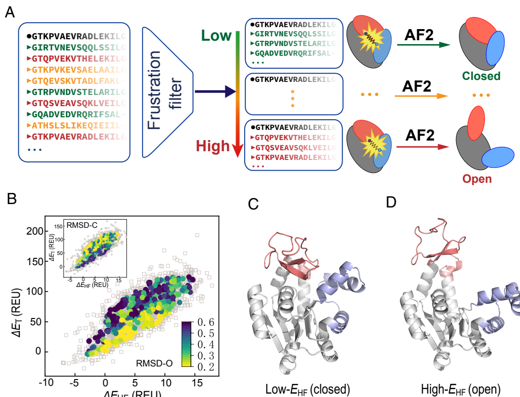
Fig. 3. Predicting alternative structures of AdK by frustration-filtering strategy. (A) The workflow of the frustration-filtering strategy in predicting protein conformational motions. (B) RMSD with respect to the reference open structure (RMSD-O, PDB code: 4AKE) for the predicted structures with the input MSA sequences taken from different locations of the two-dimensional energy space. Inset : the RMSD with respect to the reference closed structure (RMSD-C, PDB code: 1AKE). (C and D) Cartoon representations of the predicted three-dimensional structures of AdK with the low E_{HF} (C) and high E_{HF} (D) MSA sequences.
