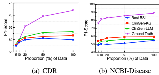
Figure 11: Different proportion of data at Base.
