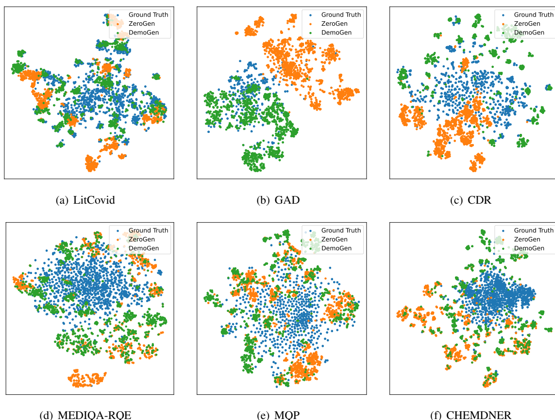
Figure 7: The t-SNE plots of datasets generated by ZeroGen and DemoGen compared with the ground truth.
