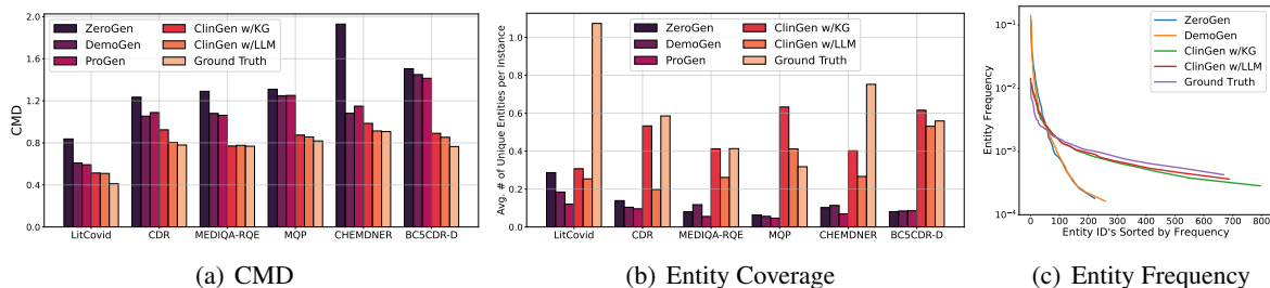
Figure 6: Data distribution and diversity measures on CLINGEN. (c) is from BC5CDR-Disease.
